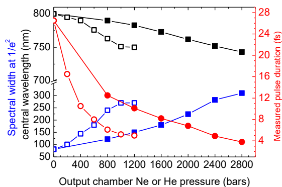
Fig 3. Spectral bandwidth, central wavelength and measured pulse duration evolution as a function of pressure in the case of Ne (open squares and circles respectively) and in the case of He (full squares and circles respectively).
