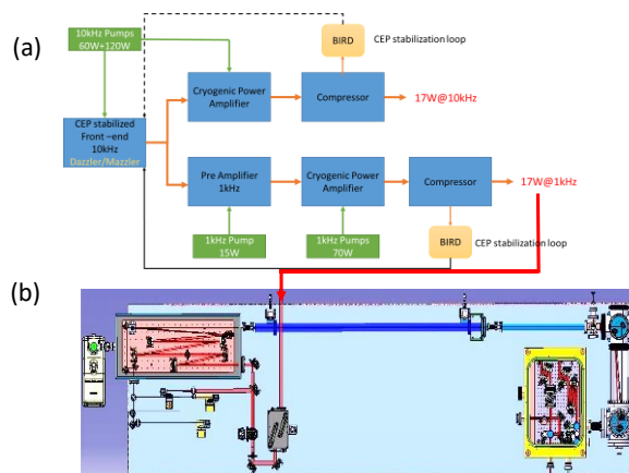
Fig 1. (a) General layout of CEP-stabilized, sub-20 fs, 1 kHz/10 kHz DUAL laser system. (b) 3D drawing of the HCF set-up with energy attenuator, coupling chamber including chirped mirrors and focusing astigmatism free telescope (in pink), output chamber with collimating telescope coupled to chirped mirror and wedges compressor (in yellow).
