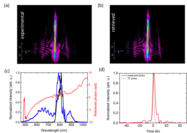
Fig 2. FROG measurement of the 2.5 mJ 1.5-cycle pulse. Panels (a) and (b) display respectively measured and retrieved FROG traces. Panel (c) displays initial (black line) and broadened (blue line) spectra with the retrieved spectral phase (red line). Panel (d) shows the retrieved temporal pulse shape (red line) and the calculated Fourier transform pulse (black dashed line).
