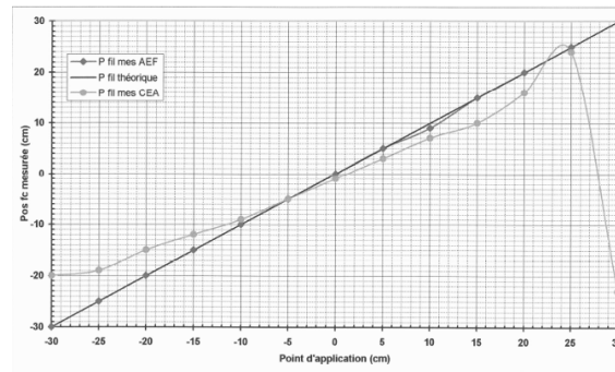
Figure 2. Sensors position calibration control procedure: computed position vs. real position.
