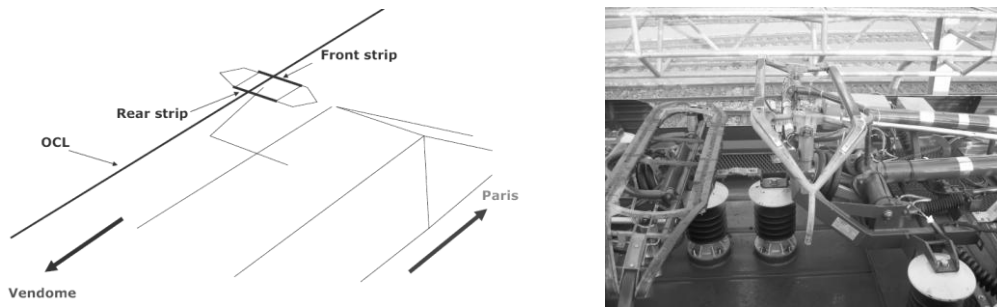
Figure 4. Pantograph configuration for Paris-Vendôme TGV field tests.
