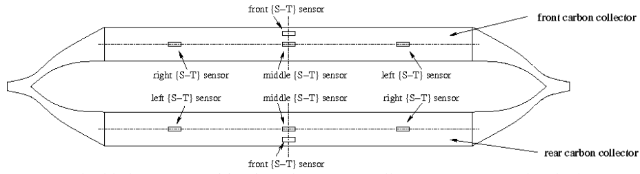
Figure 1. Embedded sensors position into the current collector (CX25 pantohead – bottom view).
