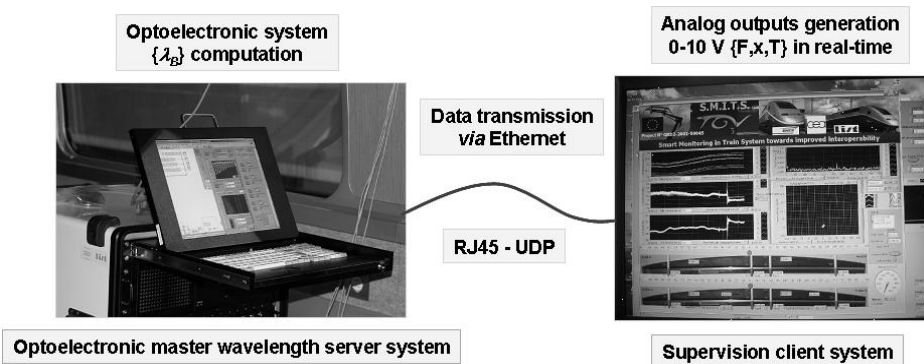
Figure 5. “Optoelectronic master” and “supervision client” monitoring system configuration.
