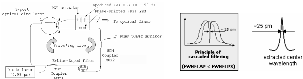
Figure 3. High scanning frequency tunable laser principle from CEA LIST.
