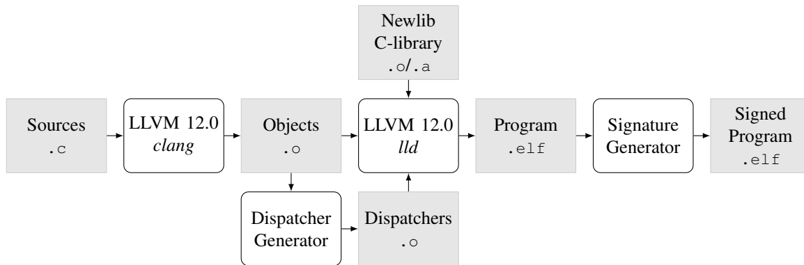
Fig. 4. MAFIA compiler toolchain with the files in light gray and the tools in rounded boxes
