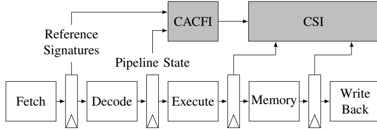
Fig. 1. Illustration of a 5-stage processor extended with MAFIA (grey modules)
