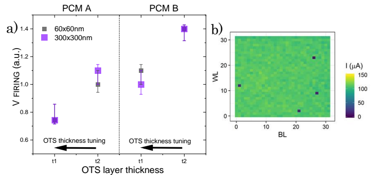
Fig. 6: a) V_{\text{FIRING}} (median values) for the different OTS thicknesses ( t_1 and t_2 ) and PCM alloys (A and B). b) Reliable firing operation at 5 V in 1 kb array of 1T1S1R 50×60 devices (based on PCM alloy A and OTS thickness = t_1 ).
