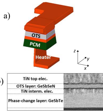
Fig. 1: a) DPSA PCM-OTS device description. b) Bright Field TEM image of the integrated stack.
