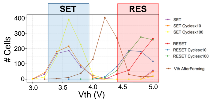
Fig. 8: SET/RESET programming in 1T1S1R 1kb arrays based on 60×80 cells. SET and RESET V_{\text{th}} distribution are reported at the starting and after 10 and 100 cycles.
