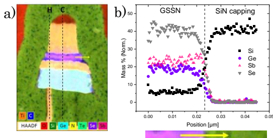
Fig. 5: a) HAADF TEM-EDX of a 60×60 device (zx plane) highlighting C/H misalignment issue. b) EDX profile performed at the OTS/SiN capping interface.
