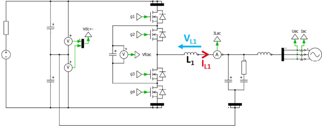
Fig. 9: PLECS simulation of the 3-phase flying capacitor inverter
