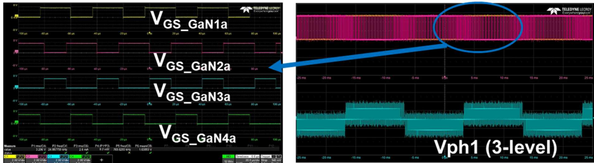
Fig. 17: Control signals of four GaN devices in a leg and the 3-level voltage of the leg
