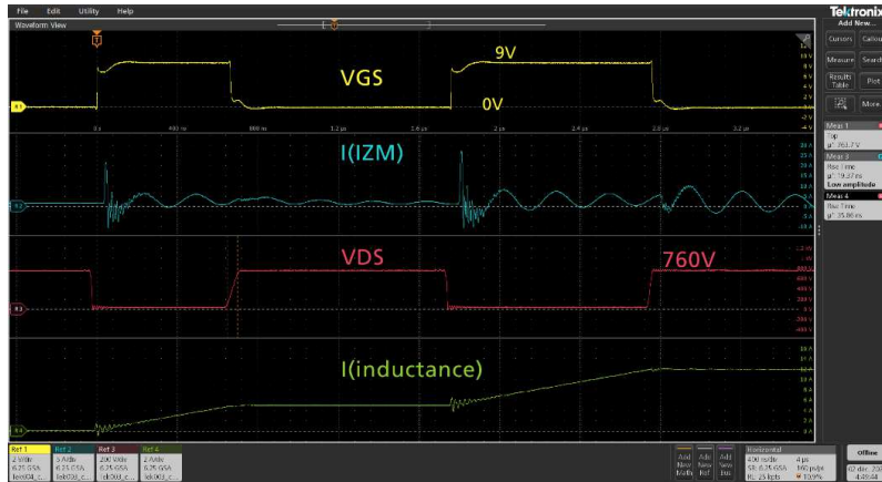
Fig. 6: Experimental waveforms of the DPT test
