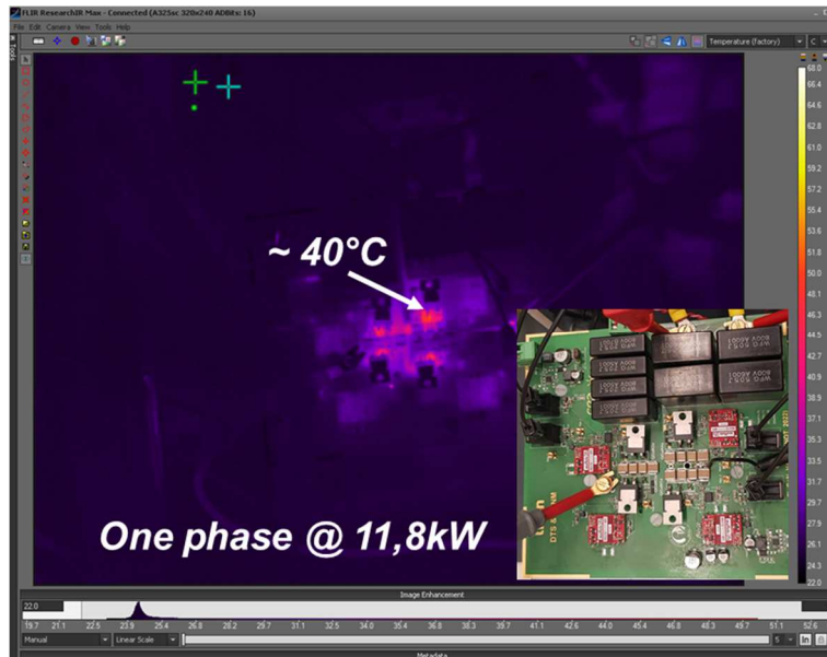
Fig. 19: Thermal image of one-phase under the output power of 11.8 kW
