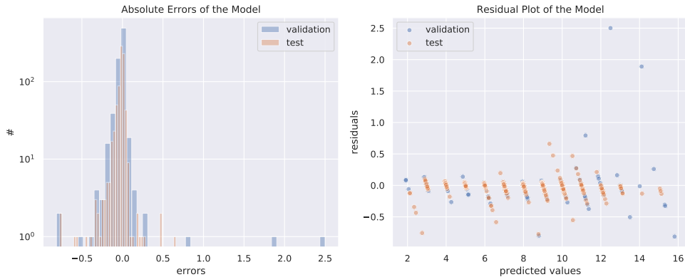
Figure 7. Difference between the true values of h^{1,1} and their predictions seen as a univariate distribution (on the left) and as a function of the predicted value (on the right): the histogram shows the distribution and extension in values of the difference between true values and predictions, while the scatter plot exhibits the constant variance of the residual error (the network performs equally well over the entire range of h^{1,1} ).
