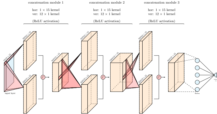
Figure 5. Schematic figure of the inception model used to predict h^{1,1} from configuration matrices.
