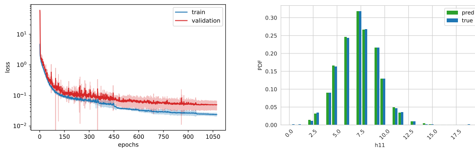
Figure 6. On the left we show the evolution of the loss evaluated on the training (blue curve) and evaluation (red curve) sets during training with 80 % training data (the colored area denotes the 1\sigma region). On the right we present the distribution of the real and predicted values for the Inception network (80 % training data).
