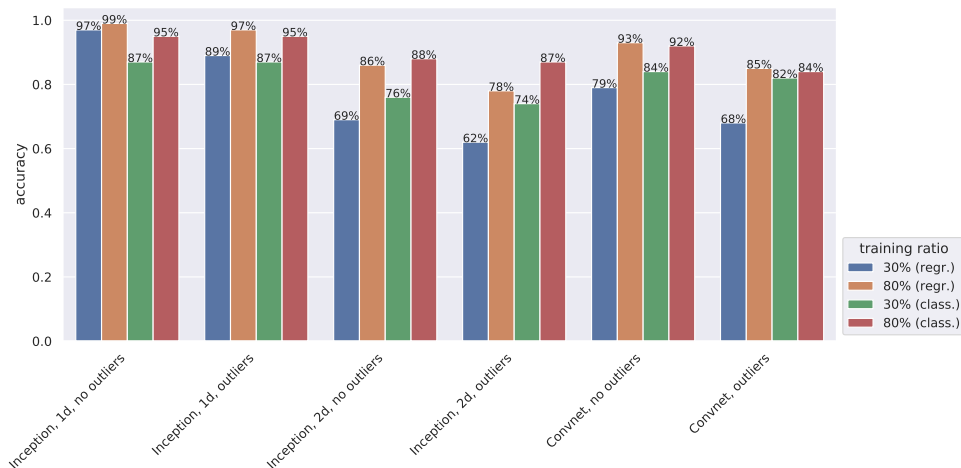
Figure 9. Comparison of accuracy for different properties. The label “no outliers” means that outliers are excluded from the training and validation set. The labels 1d and 2d refer respectively to the kernels (12 \times 1, 1 \times 15) and (3 \times 3, 5 \times 5) .
