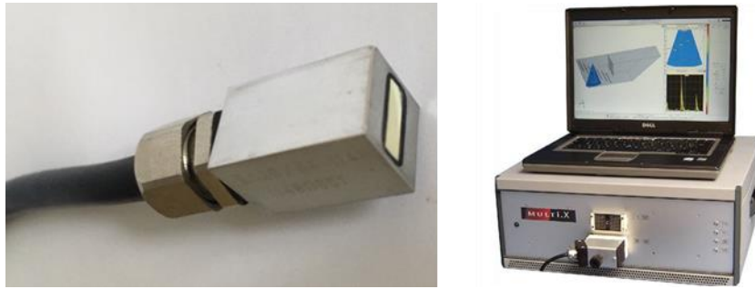
Fig. 3. Photograph of the material for ultrasonic control which was used
