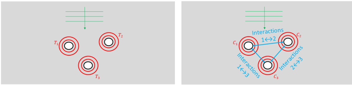
Fig. 5. Schematic representation of the difference between single (on the left) and multiple scattering (on the right) taking into account interactions
