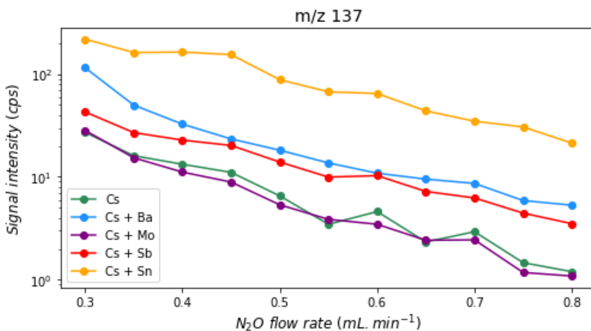
Figure S1 - Variation of signal intensities of ions with m/z 135 and 137 with N_2O flow rate for solutions containing Cs ( 10 \text{ ng}\cdot\text{mL}^{-1} ) in the presence of one measurement interferent (Mo ( 3 \text{ ng}\cdot\text{mL}^{-1} ), Sb ( 0.5 \text{ ng}\cdot\text{mL}^{-1} ), Sn ( 50 \text{ ng}\cdot\text{mL}^{-1} ) or Ba ( 5 \text{ ng}\cdot\text{mL}^{-1} ).
