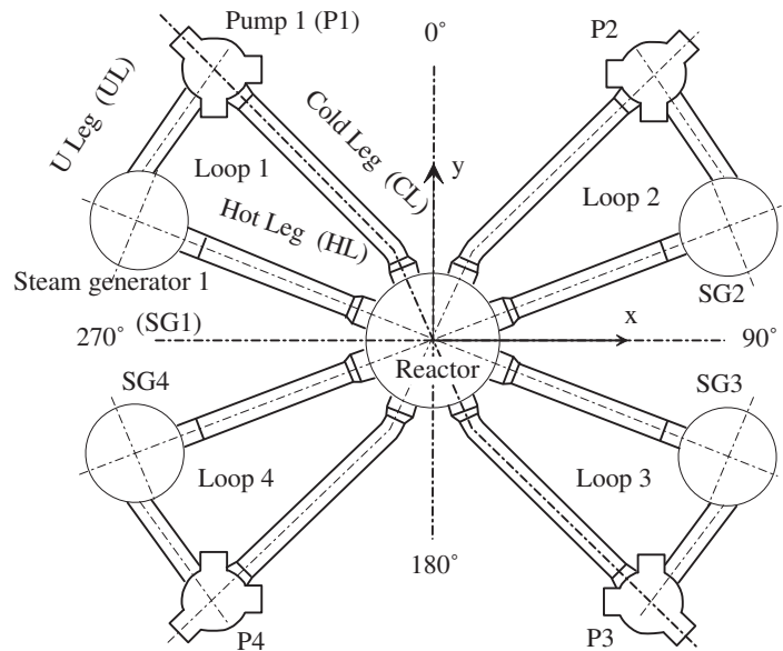
Figure 2: The primary circuit (top view)
