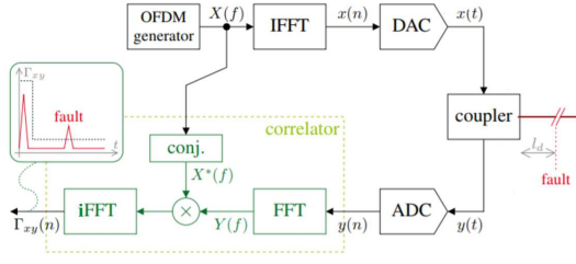
Figure 10: Schematic diagram of an OMTDR reflectometry.
