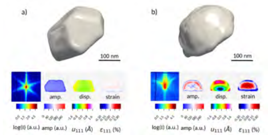
LAMMPS simulations: (a) faceted and (b) core-shell
