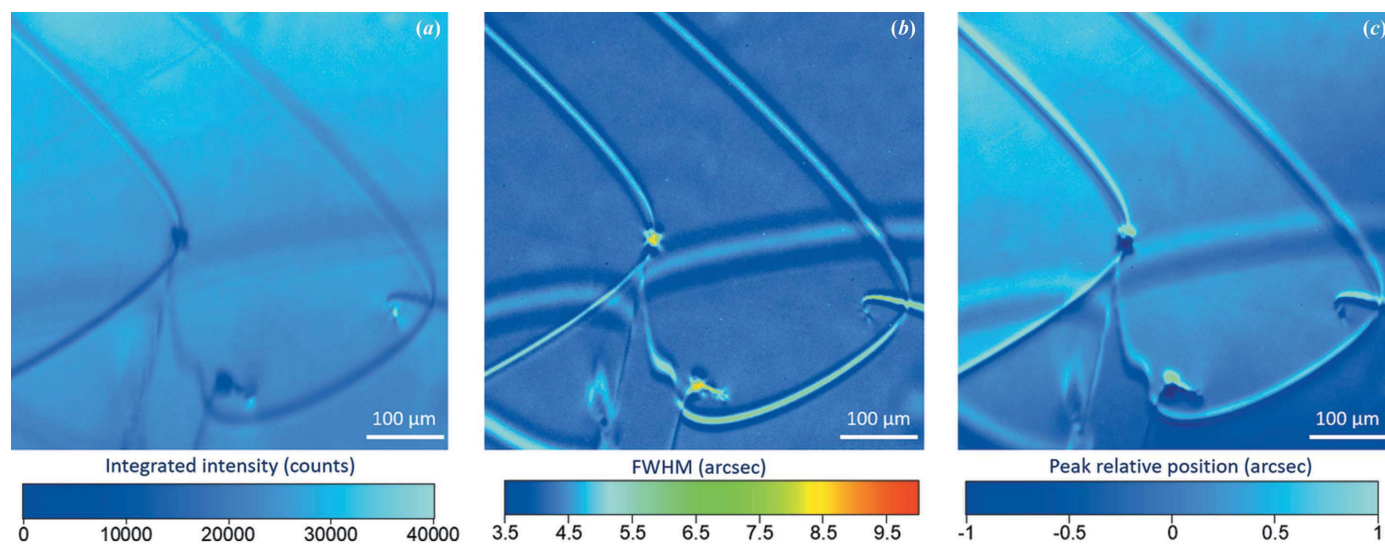
Figure 4 RCI maps of the region of the crystal imaged in Fig. 2, extracted from the rocking curves recorded on each of the pixels of the detector: (a) integrated intensity map (b) FWHM map (c) peak position map.
