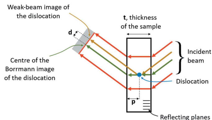
Figure 7 Schematic that considers the case of a dislocation line horizontal and parallel to the main surfaces, i.e. perpendicular to the plane of the drawing. In this case, the three-dimensional problem involving the Borrmann prism (which has, as its base, the Borrmann triangle, and the length of the horizontal extension of the beam as height) reduces to a two-dimensional problem. The drawing allows the extraction of a very simple relationship between d , the distance on the detector between the Borrmann and weak-beam images of the dislocation, and p , the distance to the exit surface.
