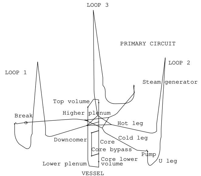
Figure 1: Pipe-model of a 3-loop PWR
