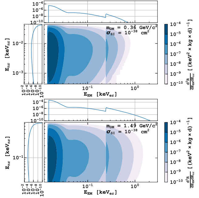
FIG. 1. 2D differential ionization rate as a function of the nuclear recoil energy ( E_{nr} ) and electromagnetic channel energy ( E_{EM} ) is shown for two representative DM masses, 0.36 \text{ GeV}/c^2 (top) and 1.49 \text{ GeV}/c^2 (bottom). The rate is given in events/( \text{keV}^2 \text{ kg d} ) and covers E_{EM} from 0.01 to 3 \text{ keV} and E_{nr} from 4 \times 10^{-4} to 4 \times 10^{-2} \text{ keV} for a DM mass of 0.36 \text{ GeV}/c^2 and E_{nr} from 2.5 \times 10^{-2} to 7.5 \times 10^{-1} \text{ keV} for a particle of mass 1.49 \text{ GeV}/c^2 . The top and side panels of each figure depict the corresponding integrated distributions in the ME electron (top panels) and the NR (left panels) channels.
