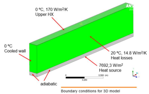
FIGURE 12: Boundary conditions in BALI-8U considered by SSTC NRS. h_{eq}=113 W/m 2 /K.
