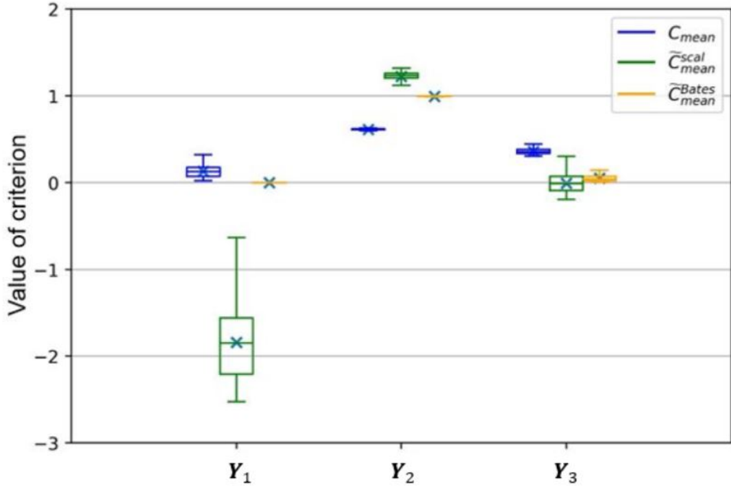
Figure 4: Boxplot of the multidimensional likelihood-based criteria C_{mean} , \widetilde{C}_{mean}^{scal} and \widetilde{C}_{mean}^{Bates} for the 3 different groups of outputs, computed on the sample of \mathcal{M}_{NuclMat} simulations. Empirical mean and median are indicated by a cross and a horizontal line, respectively.
