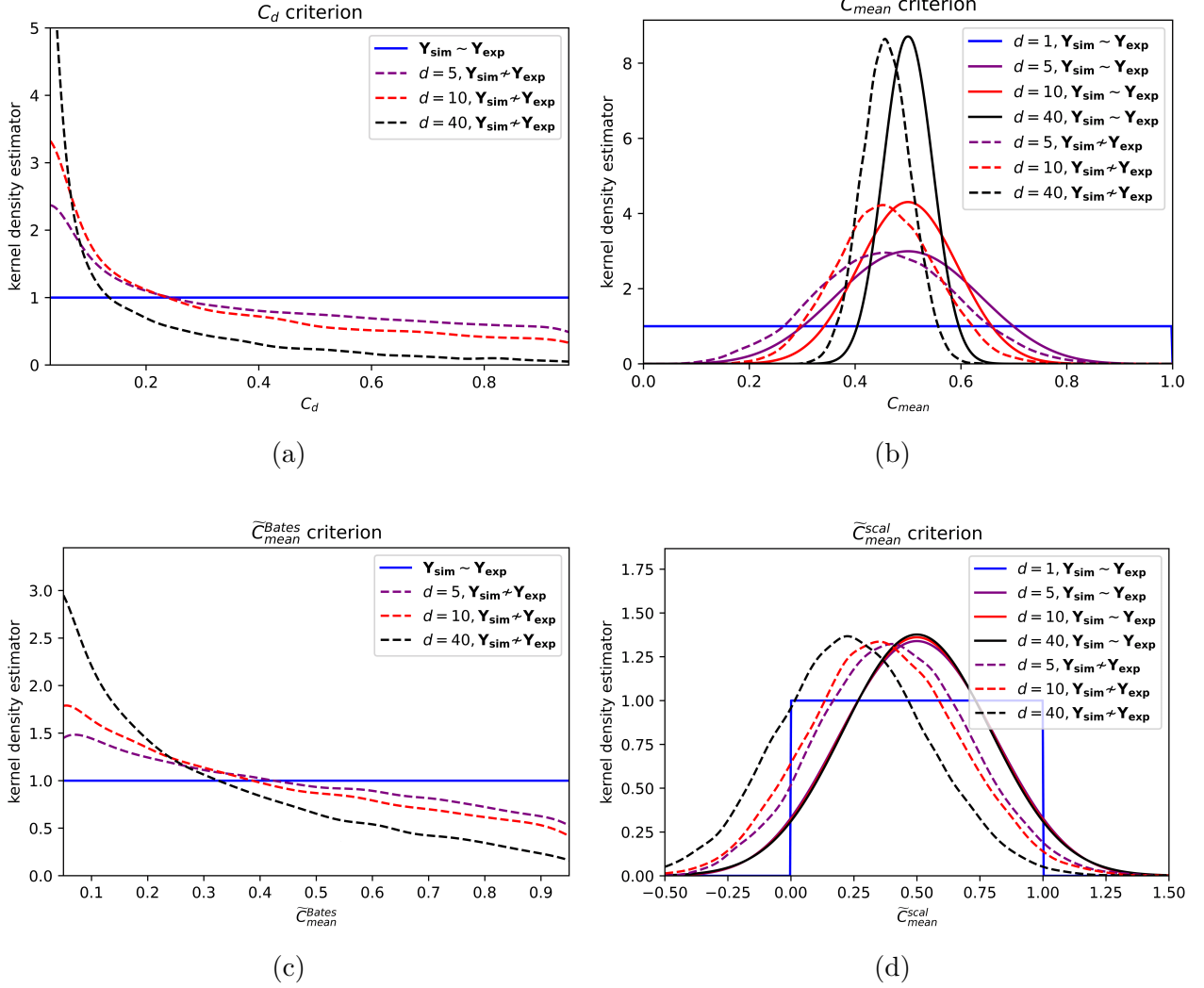
Figure 1: Estimated PDF of likelihood-based multivariate criteria for dimensions d = 5 to 40, and \mathbf{Y}_{\text{exp}} \sim N_d(\mathbf{0}, I_d) . The reference case \mathbf{Y}_{\text{sim}} \sim \mathbf{Y}_{\text{exp}} is plotted in solid lines. The case where \mathbf{Y}_{\text{sim}} also follows a d -normal distribution but with a different standard deviation on 20% of the components is plotted in dotted lines. The criteria represented here are C_d (Eq. 6), C_{\text{mean}} (Eq. 7), \tilde{C}_{\text{mean}}^{\text{Bates}} and \tilde{C}_{\text{mean}}^{\text{scal}} (Eq. 8).
