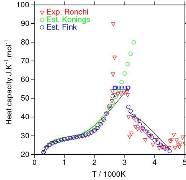
Figure 7: Heat capacity of \text{UO}_2 plotted a function of temperature using the data available in the literature [55].
