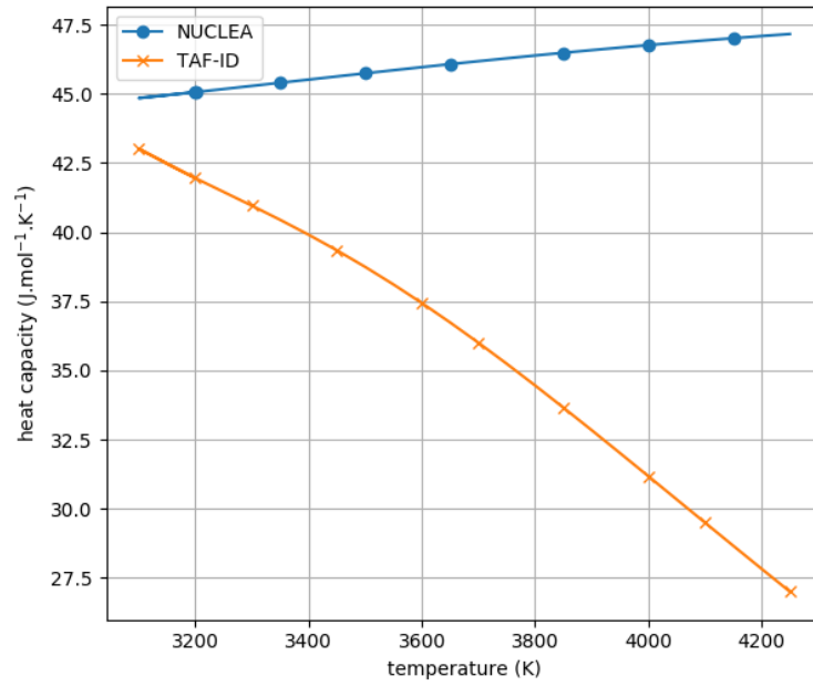
Figure 8: Heat capacity of \text{UO}_2 plotted as a function of temperature using the NUCLEA and TAF-ID databases.
