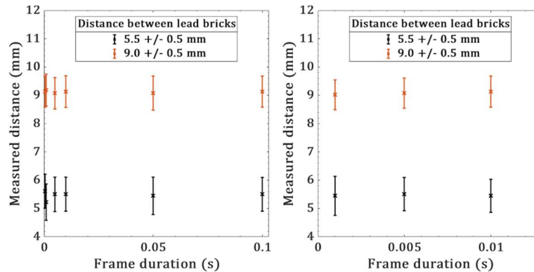
386 387 388 389 Figure 13: Measured distances between lead bricks (5.5 mm and 9 mm) with the developed system for different frame durations, for each measurements, the number of frame is 3600. Error bars are at 2 sigmas. On the left, measurements are carried out using the Cs-137 source. On the right, measurements are carried out using the Co-60.
