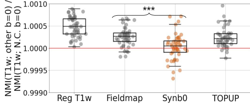
Fig. 3. Ratio between the NMI (Equation 2) calculated between T1-weighted image and b = 0 volumes obtained with each correction method and the NMI calculated between T1-weighted image and the NC b = 0 volume across the 50 subjects.
