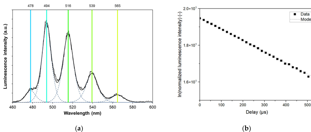
Figure 1. TRLFS results obtained at 22 °C for a solution with an initial U(VI) concentration of 5 \times 10^{-6} \text{ mol/L} in 0.8 mol/kg w \text{H}_3\text{PO}_4 : (a) U(VI) luminescence spectrum; (b) lifetime decay of the resulting U(VI) species.
