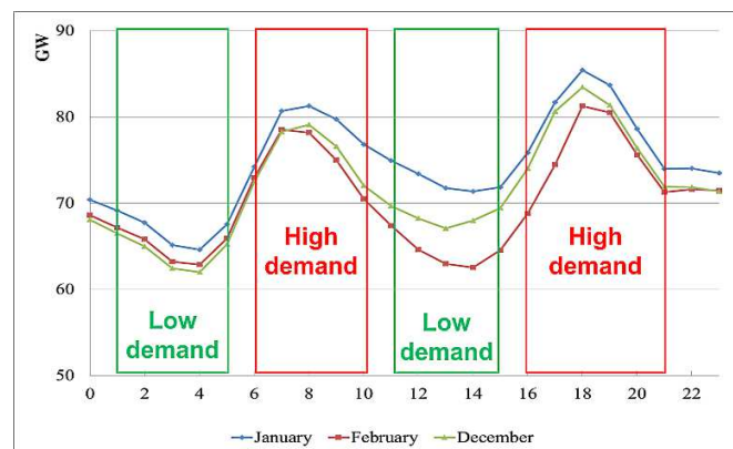
Figure 10: Example of maximum national demand for each hour of the day with PV self-consumption for December, January and February 2019
