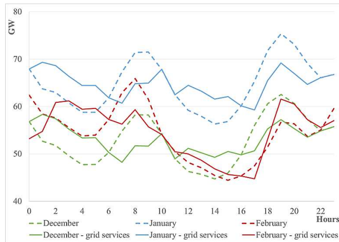
Figure 15: Grid services to smooth the daily load variation (December-January-February)
