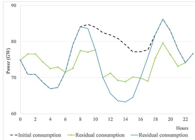
Figure 14: National consumption profiles based on the example of 24 January 2019 (peak day)
