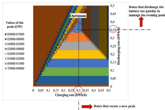
Figure 12: Results of battery charging and discharging rates obtained by the optimization loop for 2019
