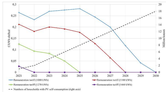
Figure 20: Sensitivity of the grid service tariffs to break-even the investment for the energy output
