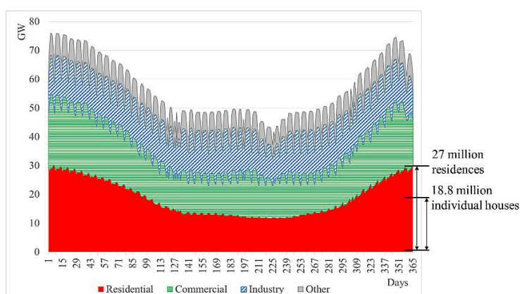
Figure 8: Annual consumption profiles by sector (2015)
