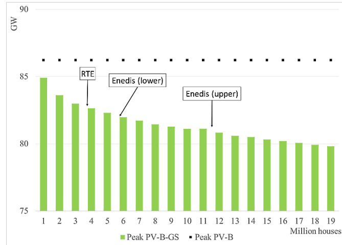
Figure 18: Sensitivity analysis of annual peak shaving impact on a national level
