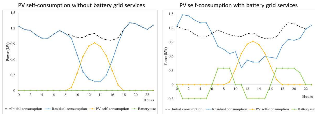
Figure 13: Residential profiles without (left) and with grid services (right): 24 January 2019 (annual peak)
