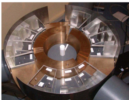
Fig. 8. The SCHEMAS bench
