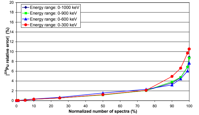
Fig. 4. Relative errors between the ^{239}\text{Pu} mass ratio obtained by IGA and the ^{239}\text{Pu} mass ratio of reference calculated for the original set of spectra with an energy range equal to 0-1 MeV and for the three sets of artificial spectra corresponding to 0-900 keV, 0-600 keV, and 0-300 keV.
