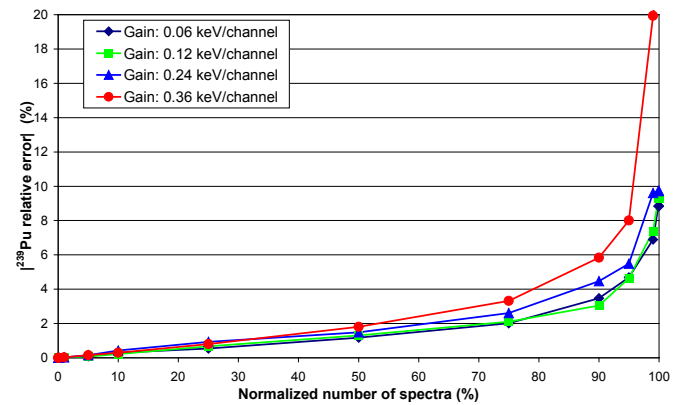
Fig. 5. Relative errors between the ^{239}\text{Pu} mass ratio obtained by IGA and the ^{239}\text{Pu} mass ratio of reference calculated for the original set of spectra with a gain equal to 0.060 keV/channel and for the three sets of artificial spectra corresponding to 0.120 keV/channel, 0.240 keV/channel, and 0.360 keV/channel.
