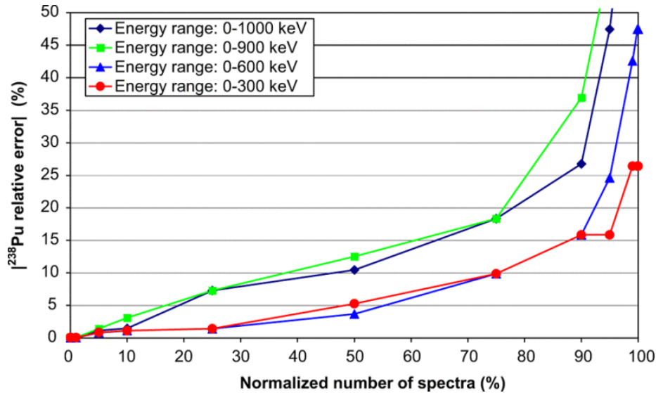
Fig. 8. Relative errors between the ^{238}\text{Pu} mass ratio obtained by IGA and the ^{238}\text{Pu} mass ratio of reference calculated for the original set of spectra with an energy range equal to 0–1 MeV and the three sets of artificial spectra corresponding to 0–900 keV, 0–600 keV and 0–300 keV.
