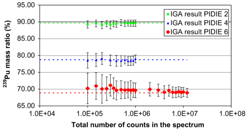
Fig. 9. IGA results for ^{239}\text{Pu} (mean of mass ratios obtained by IGA on ten or more spectra) for the three samples according to the total number of counts in the spectrum. Reference values are displayed with the dotted lines. Error bars correspond to the mean of the uncertainties provided by the code, calculated for the ten spectra of each experimental configuration.
