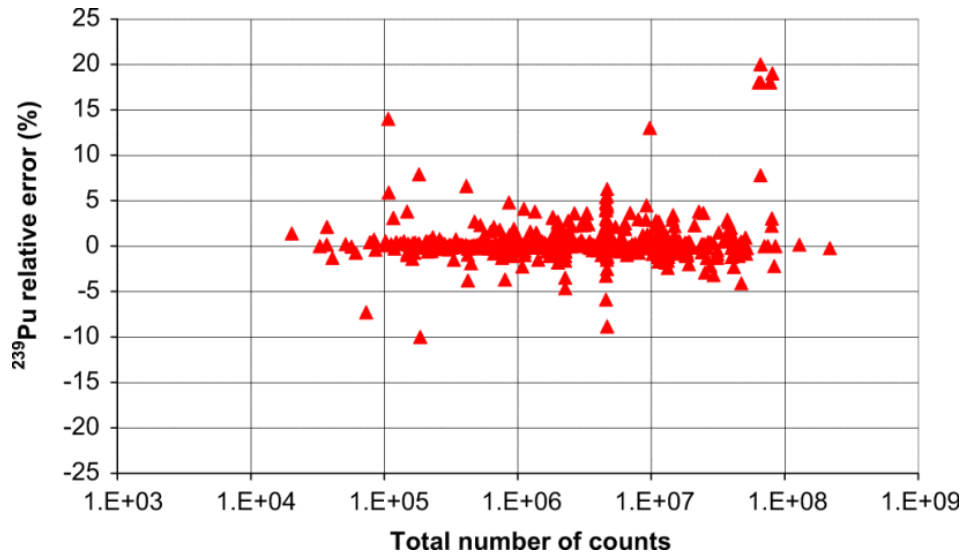
Fig. 3. Relative errors between the ^{239}\text{Pu} mass ratio obtained by IGA and the ^{239}\text{Pu} mass ratio of reference for the global Pu spectrum database according to total number of counts in the spectrum.
