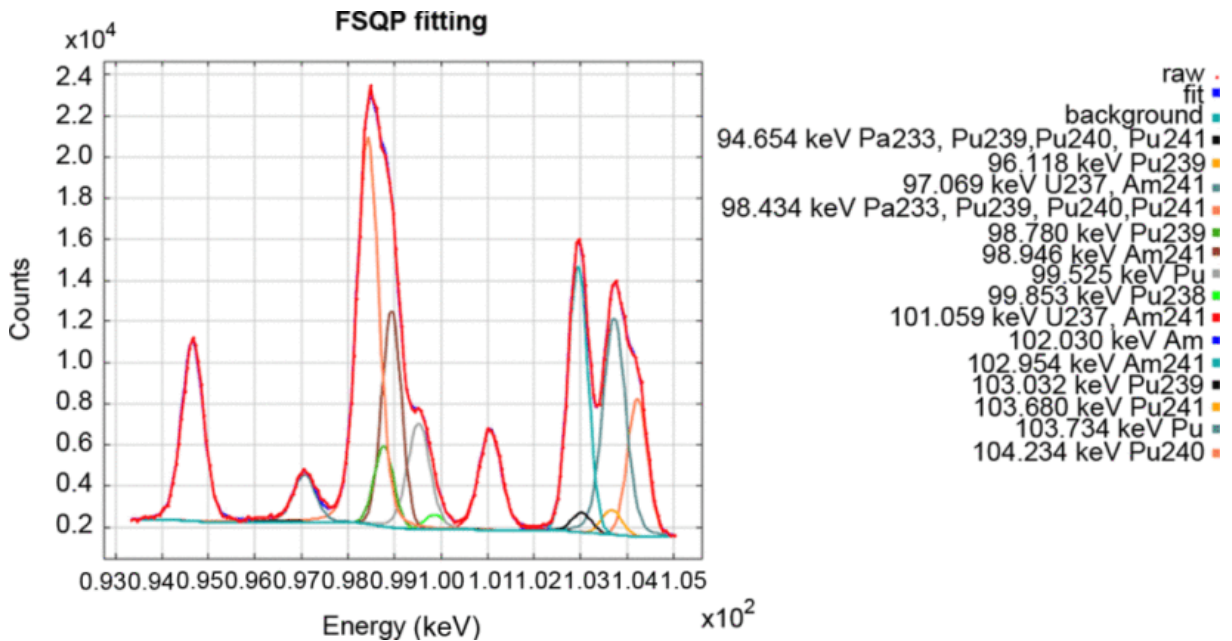
Fig. 1. Example of deconvolved region between 93 and 105 keV for a spectrum with 93.90% ^{239}\text{Pu} .
