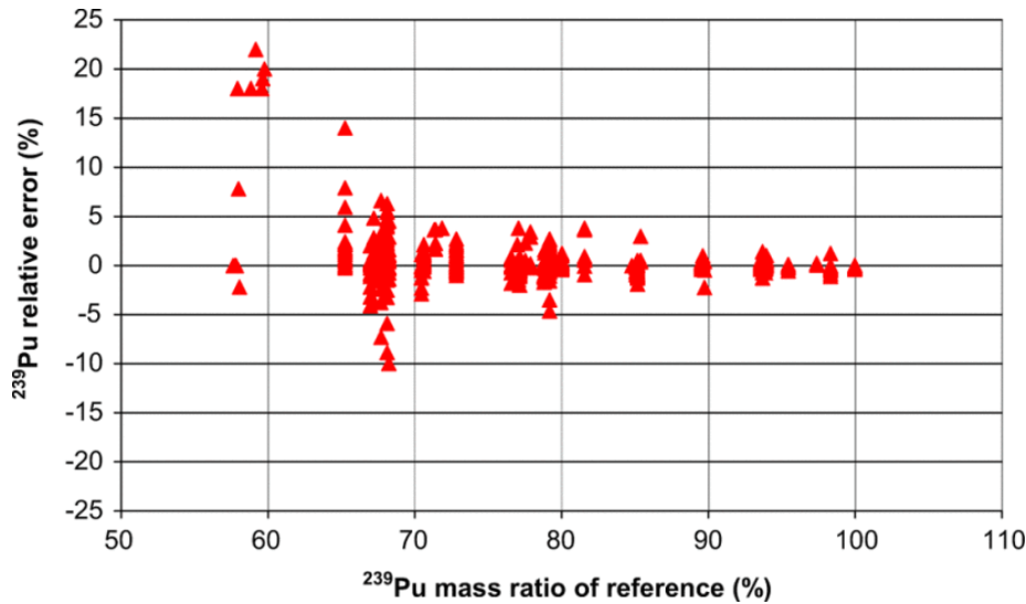
Fig. 4. Relative errors between the ^{239}\text{Pu} mass ratio obtained by IGA and the ^{239}\text{Pu} mass ratio of reference for the global Pu spectrum database according to ^{239}\text{Pu} mass ratio.
