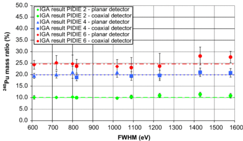
Fig. 12. IGA results for ^{240}\text{Pu} (mean of mass ratios obtained by IGA on ten or more spectra) for the three samples according to FWHM measured at 122 keV (counting statistics: 10^6 counts, gain 0.075 keV/channel). Reference values are displayed with the dotted lines. Error bars correspond to the mean of the uncertainties provided by the code, calculated for the ten spectra of each experimental configuration.
