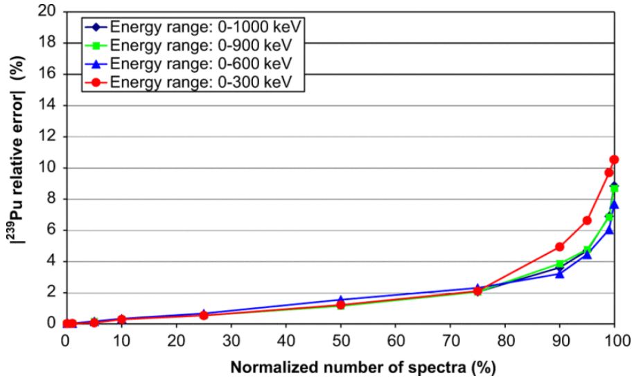
Fig. 5. Relative errors between the ^{239}\text{Pu} mass ratio obtained by IGA and the ^{239}\text{Pu} mass ratio of reference calculated for the original set of spectra with an energy range equal to 0–1 MeV and for the three sets of artificial spectra corresponding to 0–900 keV, 0–600 keV and 0–300 keV.
