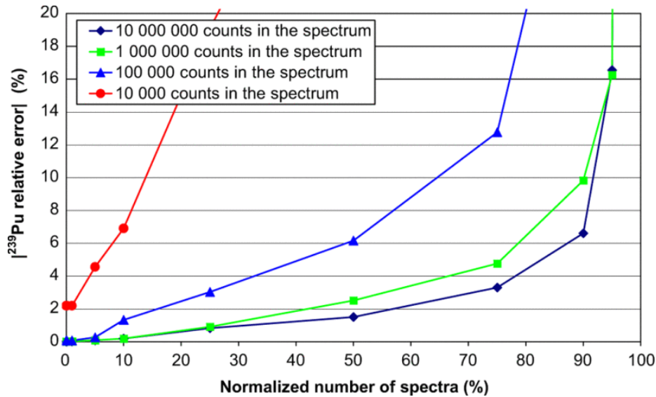
Fig. 7. Relative errors between the ^{239}\text{Pu} mass ratio obtained by IGA and the ^{239}\text{Pu} mass ratio of reference calculated for the original set of spectra with a counting statistics equal to about 10^7 counts and for the three sets of artificial spectra corresponding to 10^6 counts, 10^5 counts and 10^4 counts in the spectrum.
