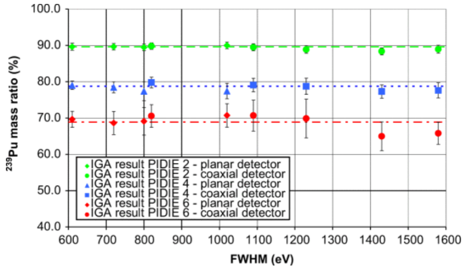
Fig. 11. IGA results for ^{239}\text{Pu} (mean of mass ratios obtained by IGA on ten or more spectra) for the three samples according to FWHM measured at 122 keV (counting statistics: 10^6 counts, gain 0.075 keV/channel). Reference values are displayed with the dotted lines. Error bars correspond to the mean of the uncertainties provided by the code, calculated for the ten spectra of each experimental configuration.
