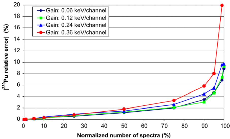
Fig. 6. Relative errors between the ^{239}\text{Pu} mass ratio obtained by IGA and the ^{239}\text{Pu} mass ratio of reference calculated for the original set of spectra with a gain equal to 0.060 keV/channel and for the three sets of artificial spectra corresponding to 0.120 keV/channel, 0.240 keV/channel and 0.360 keV/channel.
