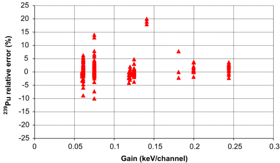
Fig. 2. Relative errors between the ^{239}\text{Pu} mass ratio obtained by IGA and the ^{239}\text{Pu} mass ratio of reference for the global Pu spectrum database according to gain.
