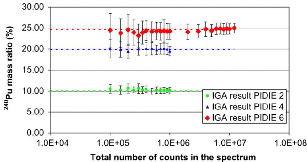
Fig. 10. IGA results for ^{240}\text{Pu} (mean of mass ratios obtained by IGA on ten or more spectra) for the three samples according to the total number of counts in the spectrum. Reference values are displayed with the dotted lines. Error bars correspond to the mean of the uncertainties provided by the code, calculated for the ten spectra of each experimental configuration.
