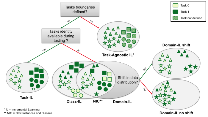
Fig. 1: Atlas of continual learning scenarios
