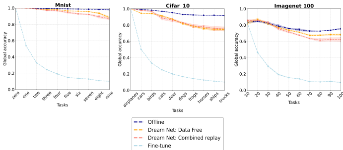
Fig. 2: Global accuracy across tasks for Class-IL incremental batch learning sub-scenario 1.A. Dream Net - Data Free is compared to baseline models and Dream Net - Combined replay model on Mnist, Cifar10 and Imagenet100
