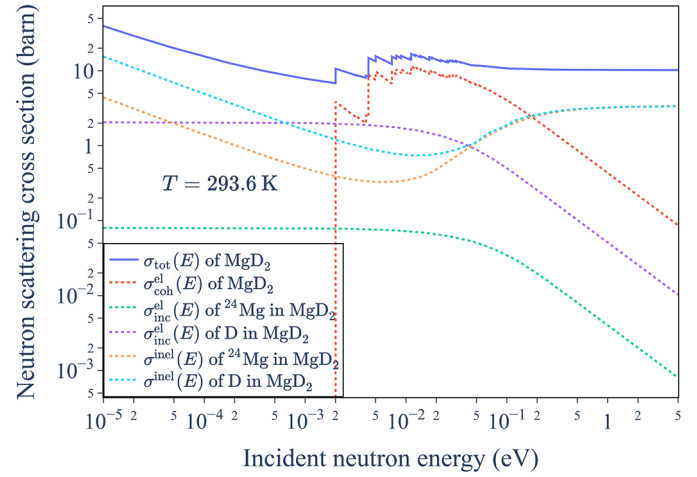
Fig. 9. Total scattering cross section (solid line) and the coherent/incoherent elastic/inelastic components (dot lines) of \text{MgD}_2 at 293.6 K.
