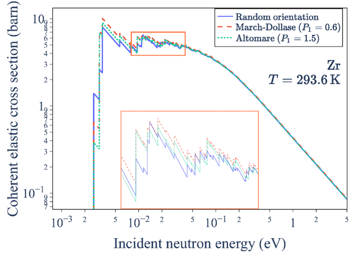
Fig. 13. Comparison of coherent elastic scattering cross section \sigma_{\text{coh}}^{\text{el}}(E) of zirconium with random orientation and with preferred orientation \vec{P}\text{O} = [0, 0, 1] . \sigma_{\text{coh}}^{\text{el}}(E) obtained by using the cylindrically symmetric PDDFs proposed by March-Dollase and Altomare et al. are respectively presented.
