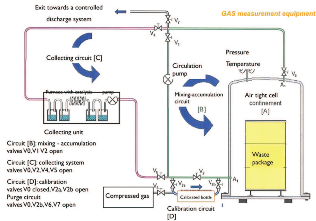
Fig. 18. Description of an accumulation measuring device.
