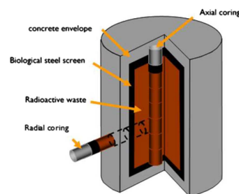
Fig. 11. Schematic diagram of core drilling.
