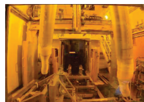
Fig. 12. Installation of an 870 l drum in CADECOL.
