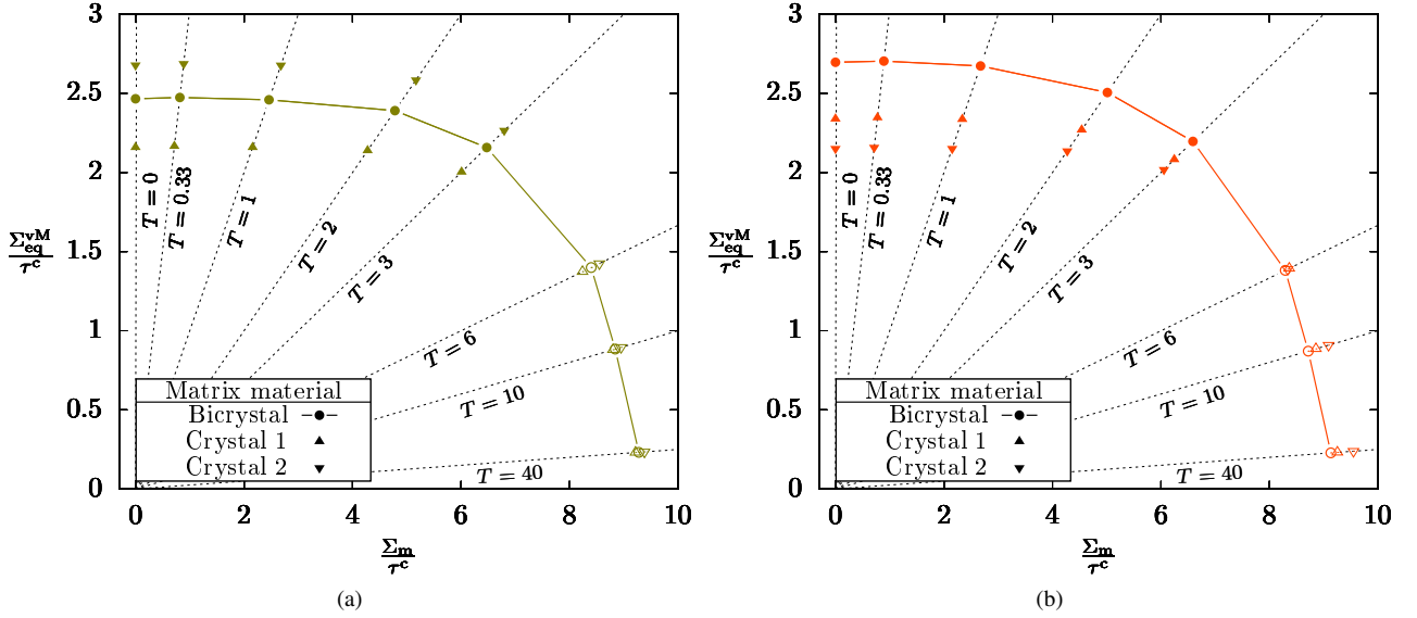
Figure 3: Yield surfaces of porous bi-crystals (Fig. 1a) and corresponding porous constitutive single crystals (Fig. 1c) at f = 0.005 , n = 100 and \theta = 0 : (a) crystal orientation couple #3; (b) crystal orientation couple #2. Hollowed-out symbols mark simulations in which the deformation mode has been identified as void coalescence.
