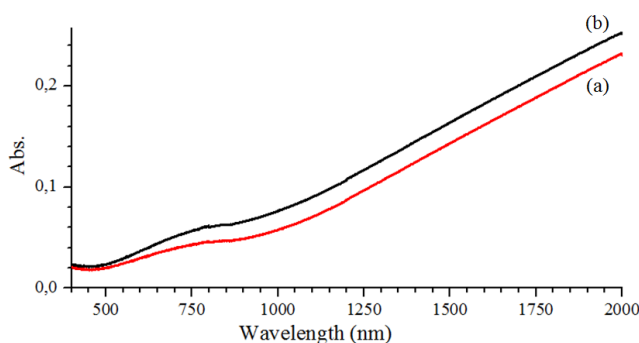
Fig. 2 UV-Vis-NIR absorbance spectra of (a) pristine PEDOT:PSS layer and (b) EG dipped PEDOT:PSS layer
