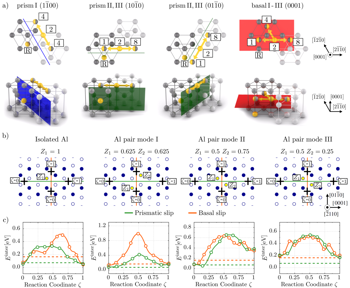
Figure 2. (a) Three geometrically possible prismatic and basal cutting modes of the second NN solute pair in \alpha -Ti. (b) Initial \zeta = 0 and final \zeta = 1 positions of 1/3(1\bar{2}10) screw dislocation gliding next to isolated Al atom or cutting the second NN Al pair along prismatic and basal modes I–III. Z_1 and Z_2 indicate the position (normalized by the lattice parameter a ) of solute atoms along dislocation line in the simulation box. Ti atoms belonging to different (\bar{2}110) are plotted with open or full-colored circles. Solute atoms are denoted by yellow color. The corresponding minimum energy paths of particular prismatic and basal slip modes are given in (c), with the Peierls energy barriers of pure Ti marked by dashed lines.
