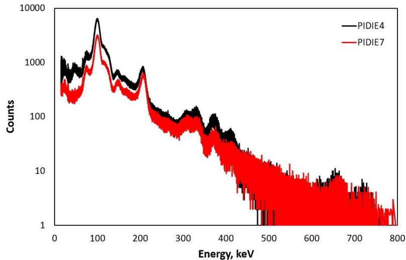
Figure 6: Plutonium spectra measured on a TimePix3 CdTe detector.
