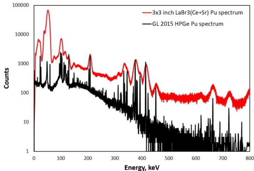
Figure 3: Spectrometric performance comparison of 3x3 inch LaBr 3 (Ce+Sr) and GL 2015 HPGe detectors.
