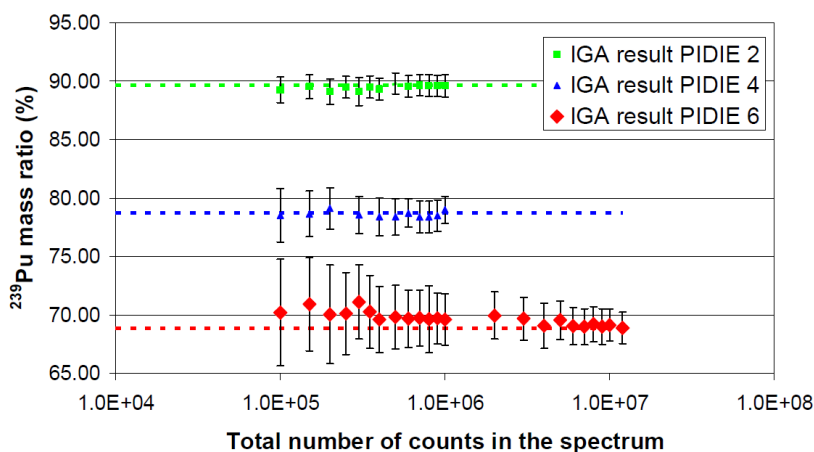
Figure 1: Impact of the counting statistics on the IGA code performance with Pu samples of different isotopic composition [37].
