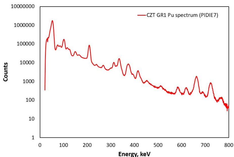
Figure 5: Plutonium spectrum measured on a CZT-based GR1 detector by Kromek.
