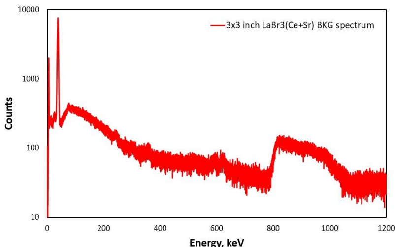
Figure 4: Background radiation spectrum measured on a 3x3 inch LaBr 3 (Ce+Sr) detector.
