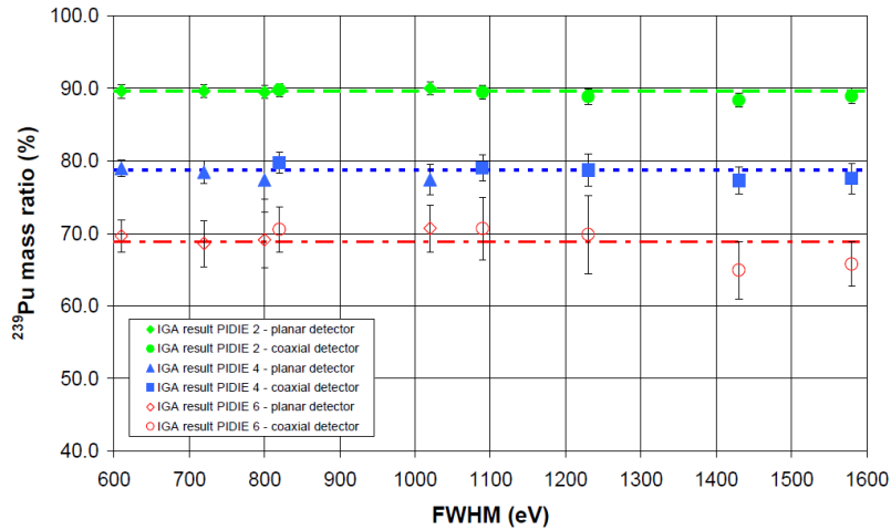
Figure 2: Impact of the detector energy resolution on the IGA code performance with Pu samples of different isotopic composition [37].
