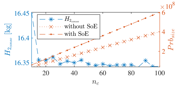
Fig. 5: PMS sensitivity to n_c
