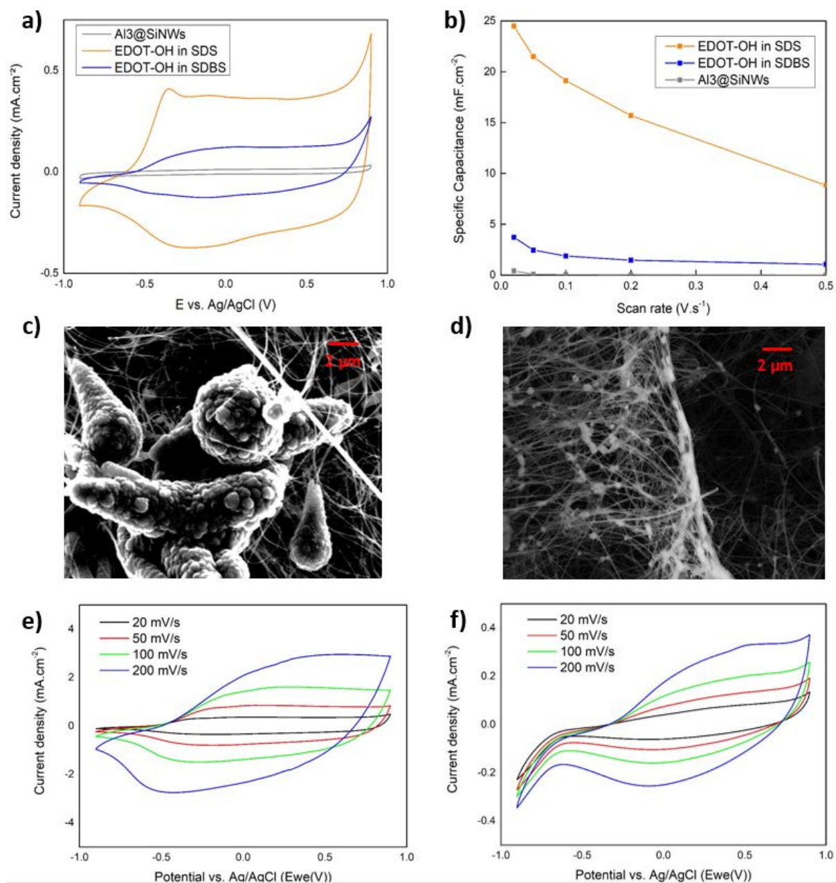
Figure 3. (a) Comparison between with the bare \text{Al}_3\text{@SiNWs} of the SDS and SDBS 100 cycles electropolymerization in \text{Na}_2\text{SO}_4 0.7 M and (b) their capacitance evolution regarding the scan rate. SEM images of electropolymerization made with (c) SDS and (d) SDBS in SE2. Cyclic voltammetry at different scanning rate of (e) EP in SDS and (f) EP in SDBS.
