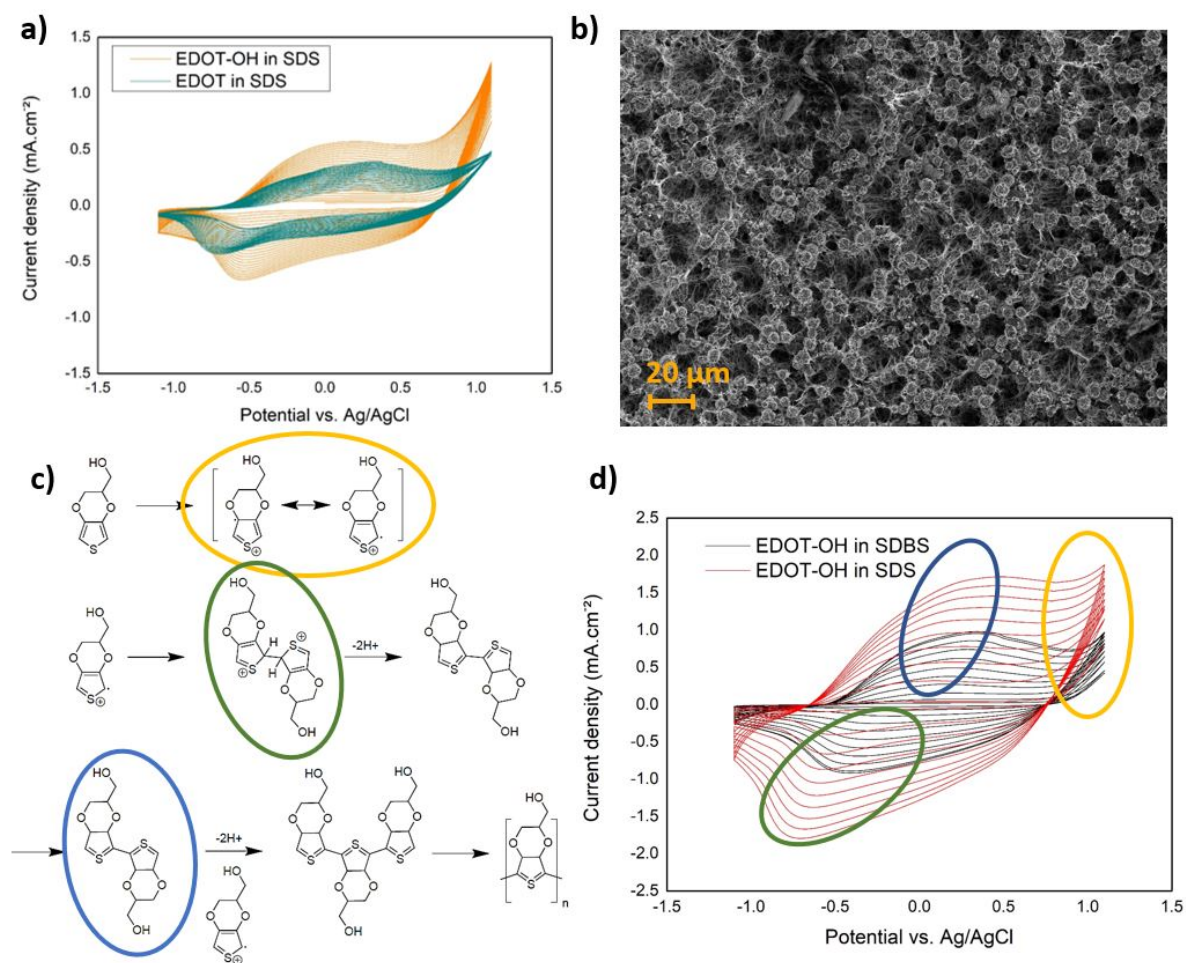
Figure 1. Nanocomposite electrode formulation, with (a) the electropolymerization comparison of EDOT and EDOT-OH, (b) the SEM top view of the PEDOT-OH-Al 3 @SiNWs nanocomposite electrode, (c) electropolymerization mechanism described and main deposition steps specified on the CV curves, with circled in yellow the polaronic form, circled in green the dimerization, circled in blue the propagation of the phenomenon and deposition of polymer EDOT-OH (d) comparison of surfactants SDS and SDBS in electrodeposition of EDOT-OH at 50 mV·s -1 , critical micellar media (0.01 M).
