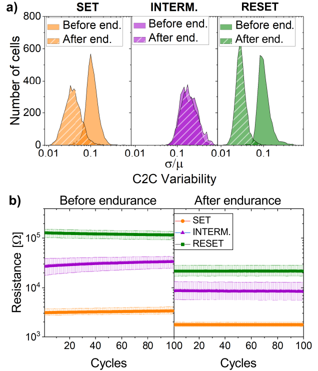
Fig. 11. Variability of SET, RESET and intermediate states evaluated along 100 programming cycles (SET/RESET pulses of 50 ns) in TiTe/GST 4 kb arrays, before and after an endurance test compatible with the one performed in Fig. 8. a) C2C variability distributions: for each device in the array the C2C variability was calculated as the ratio between the standard deviation of the resistance value and its median resistance along 100 cycles. b) D2D variability: median and standard deviation for the 4 kb resistance values along the 100 cycles.
