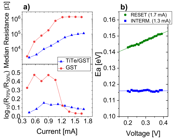
Fig. 6. a) Intermediate states obtained in GST and TiTe/GST applying 300 ns squared pulses with increasing current intensity pre-programming the array in the SET state before each pulse. Median (above) and variability (below) of the resistances in 4 kb arrays are represented. The variability was calculated as the ratio between the 70th and the 30th percentile of the 4 kb resistances. b) Activation energy of the conduction measured from I-V characteristics of TiTe/GST (not reported), for RESET state and an intermediate state, following the model from [8].
