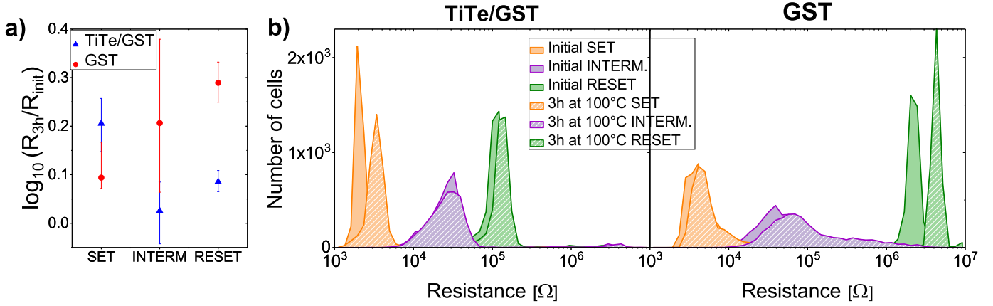
Fig. 7. Data retention evaluated after annealing at 100^{\circ}\text{C} for the SET, intermediate and RESET states in TiTe/GST and GST 4 kb arrays. a) The resistance drift is quantified as the ratio between the resistance measured after a 3 hours annealing and the initial resistance. Median values and variability are represented. b) Resistance distributions of the three states before and after 3 hours annealing at 100^{\circ}\text{C} .
