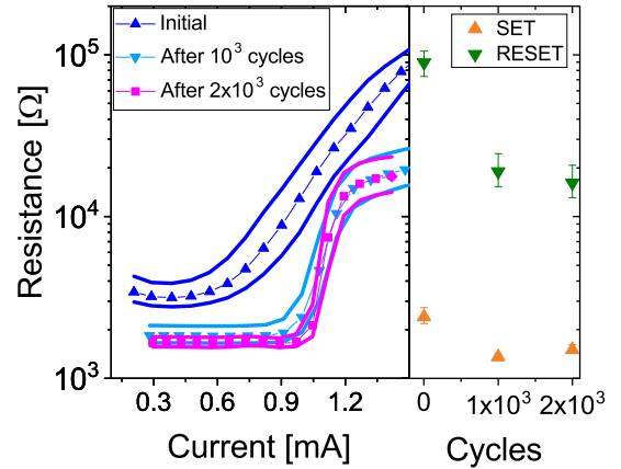
Fig. 8. Left: R-I characteristic at the beginning of the devices life and after endurance for TiTe/GST. Right: 4 kb TiTe/GST SET and RESET resistances evolution along cycles performed with pulses of 10\ \mu\text{s} to accelerate and evidence the evolution.
