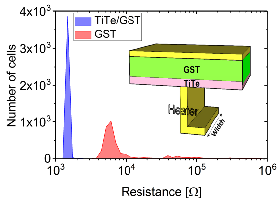
Fig. 2. As-fabricated resistance distributions of TiTe/GST and GST 4 kb arrays. Inset: simplified scheme of the studied "Wall" PCM device based on TiTe/GST bi-layer stack.
