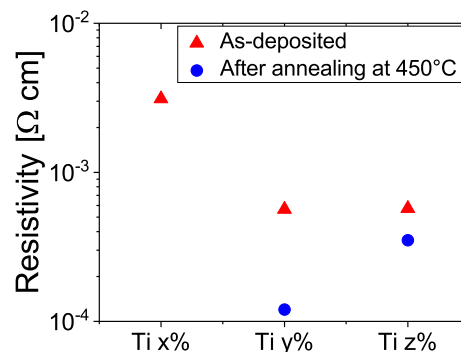
Fig. 1. Resistivity of TiTe samples with three different percentages of Ti (x, y and z with x < y < z ) measured at room temperature before and after annealing at 450°C. The resistivity after annealing of the layer with Ti x % is not reported since the layer resulted degraded after the test.
