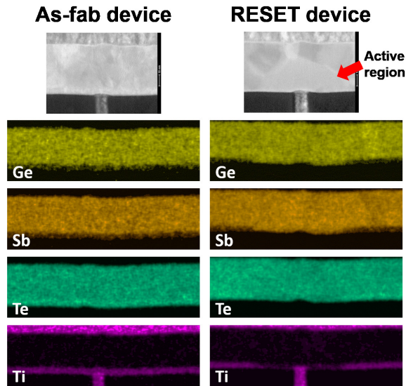
Fig. 3. TEM/EDX analyses performed on as-fabricated TiTe/GST device (left column) and on a device programmed in the RESET state after initialization (right column).
