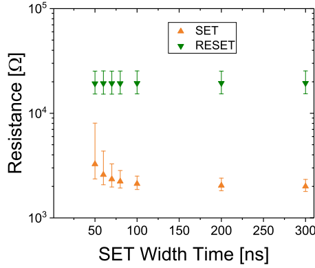
Fig. 9. SET speed test realized in TiTe/GST 4 kb array after endurance test performed in Fig. 8b, using SET pulses with increasing width time and short constant fall time of 10 ns.
