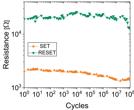
Fig. 10. Endurance evaluated in a TiTe/GST device with optimized SET and RESET pulses (width time = 50 ns, rise/fall time = 10 ns).
