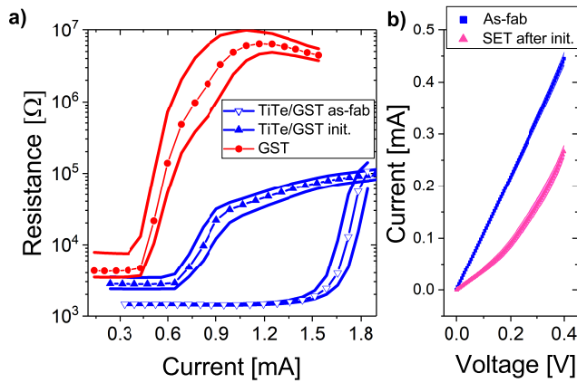
Fig. 4. a) Resistance as a function of current measured in 4 kb array for GST and TiTe/GST devices starting in the SET state. We represent median values and 1\sigma intervals, and in particular before (as-fab) and after initialization (init.) for TiTe/GST. b) Current-Voltage (I-V) characteristics of five TiTe/GST PCM devices as-fabricated (as-fab) and after initialization in the SET state (SET after-init.).
