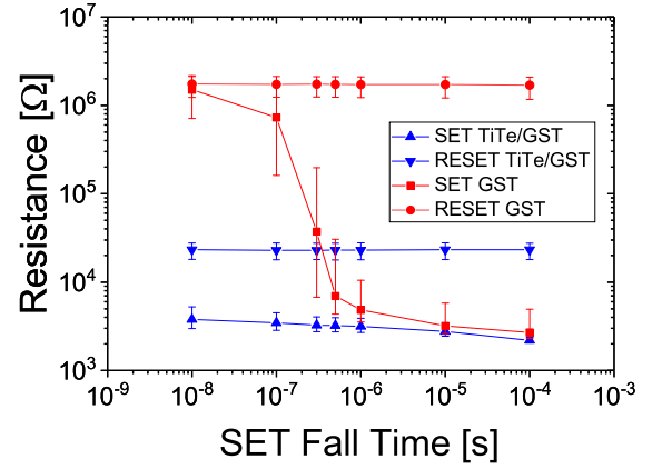
Fig. 5. SET speed test performed on TiTe/GST and GST 4 kb arrays. Data are obtained applying a SET pulse with optimized current, 300 ns width time and incremental fall time on arrays pre-programmed in RESET state before each SET pulse. RESET state resistance is reported as well.
