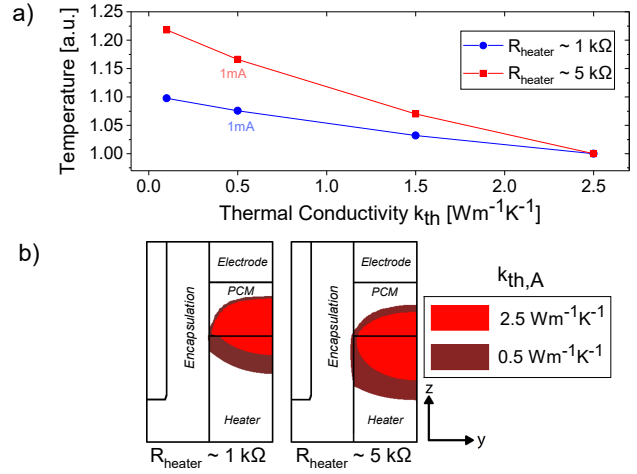
Fig. 8. a) Evolution of the maximum temperature reached inside the chalcogenide material in the PCM cell, depending on the thermal conductivity of the dielectric A ( k_{th,A} ) and for two different values of heater resistance. Temperature is normalized and is obtained from equivalent programming currents. b) Temperature profile (region that during RESET current application achieves a temperature higher than 930 K) achieved in the two devices for a low and a high thermal conductivity dielectric A. Based on the same maximum temperature obtained for k_{th,A} = 2.5 \text{ Wm}^{-1}\text{K}^{-1}
