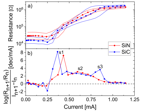
Fig. 4. RI characteristics for both SiN and SiC 4kb PCM arrays, obtained with staircase protocol (pulse width = 300 ns, fall-time = 10 ns). Median resistance with 15%-85% confidence interval is reported as a function of the programming current (a), associated with the evolution of the slope s of each curve (b).
