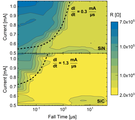
Fig. 5. SET resistance cartographies as a function of the programming current and of the duration of the falling edge of the SET pulse (pulse width kept constant at 300 ns). Median values from 30 cells with 100 nm heater width are reported. Dashed lines represent the current over fall-time rate necessary to achieve the SET state in both SiC and SiN (SET state = 10% of the Resistance window).
