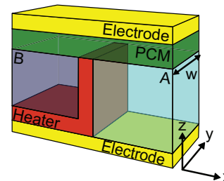
Fig. 1. Description of a “Wall” PCM device. The dielectrics integrated on the two sides of the heater are named respectively A (SiN or SiC) and B (SiN).
