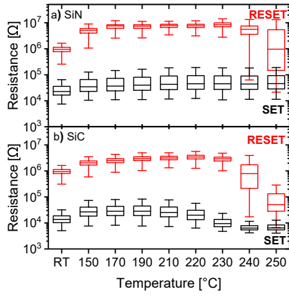
Fig. 7. Data retention tests performed by isochronal annealing of 1 hour at increasing temperatures for SiC and SiN devices.
