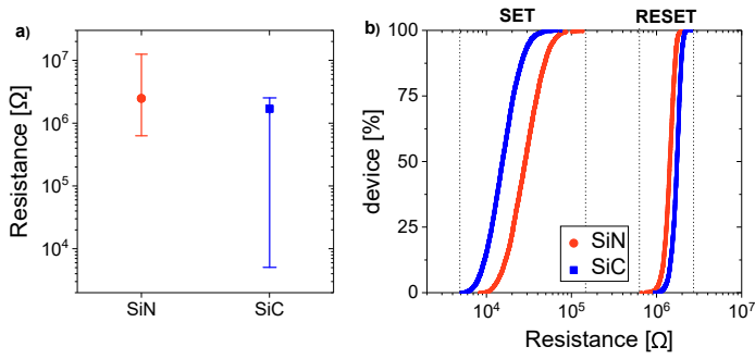
Fig. 2. a) Median virgin resistance with error bars defined as minimum and maximum values. b) Cumulative distributions in the 4kb array of the SET and RESET resistance states after initialization, for both SiC and SiN-PCM.
