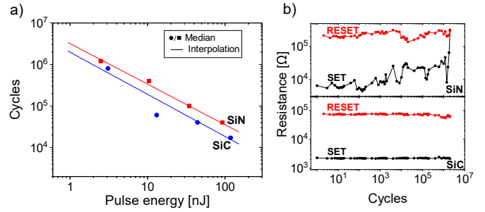
Fig. 6. a) Median (based on 25 devices) of the number of cycles until failure as a function of the total energy of the SET+RESET programming, modulated by varying the width of the SET and RESET combination of pulses. Lines are linear regressions of the data. b) Example of endurance tests performed with same programming conditions for SiN and SiC PCM.
