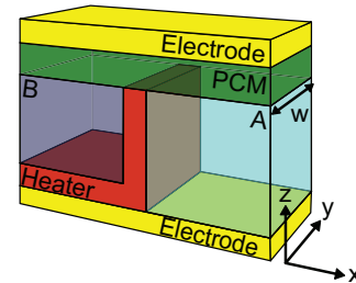
Fig. 1. Description of a “Wall” PCM device. The dielectrics integrated on the two sides of the heater are named respectively A (SiN or SiC) and B (SiN).
