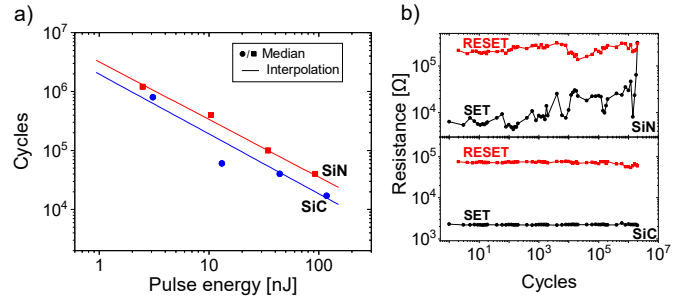
Fig. 6. a) Median (based on 25 devices) of the number of cycles until failure as a function of the total energy of the SET+RESET programming, modulated by varying the width of the SET and RESET combination of pulses. Lines are linear regressions of the data. b) Example of endurance tests performed with same programming conditions for SiN and SiC PCM.
