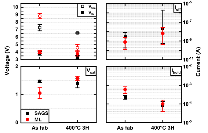
Fig. 5. Electrical parameters measured in AC (at the exception of I_{off} measured in DC) on devices as-fabricated and annealed for 3 hours at 400°C. The close electrical behavior of ML and SAGS, is likely related to the same features (i.e. AsSe) responsible for the switching mechanism in both materials.
