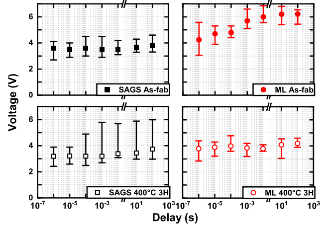
Fig. 6. V_{th} drift measured on as-fabricated and annealed devices. The defects related to Ge-Ge bonds owing to GeN layer in ML, present in As-fab devices, relax in time causing an important drift. After annealing, SAGS exhibits a median low drift affected by a 3 V spread while ML shows lower drift (with respect to As-fab ) and low variability.
