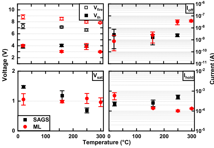
Fig. 4. Electrical parameters V_{fire} , V_{th} , V_{sat} and I_{hold} measured by AC protocols and I_{off} measured by DC voltage application (at V_{th}/2 ), from room temperature up to 250°C for SAGS and up to 300°C for ML. SAGS devices do not show functionality at 300°C.
