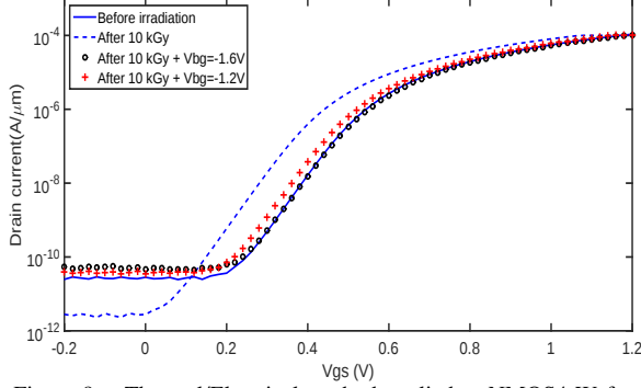
Figure 9. Thermal/Electrical method applied to NMOS4 Wafer 2.
