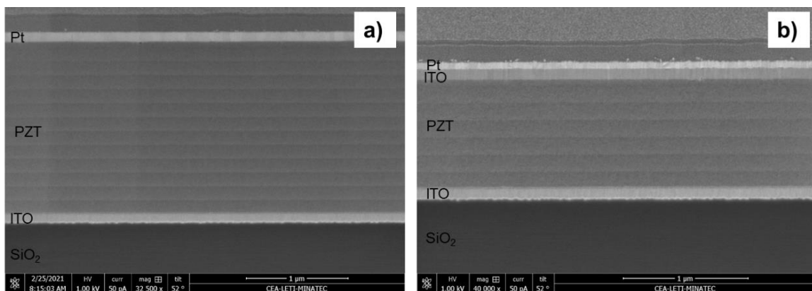
Fig. 3. FIB-SEM images of a) Pt/PZT 2 \mu\text{m} /ITO after transfer and b) Pt/ITO/PZT 1 \mu\text{m} /ITO stack.
