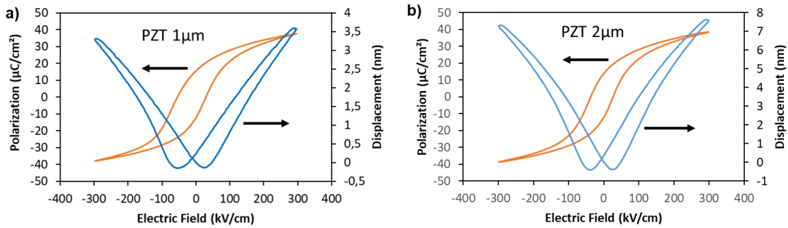
Fig. 6. Polarization and displacement as a function of electric field for a) PZT 1 \mu\text{m} and b) PZT 2 \mu\text{m}
