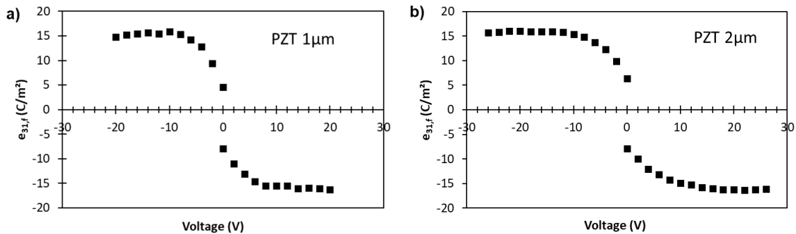
Fig. 7. Piezoelectric coefficient e_{31,f} as a function of applied voltage for a) PZT 1 \mu\text{m} and b) PZT 2 \mu\text{m}
