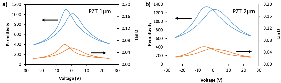
Fig. 5. Dielectric permittivity \epsilon_r and losses \tan \delta as a function of voltage for a) PZT 1 \mu\text{m} and b) PZT 2 \mu\text{m}
