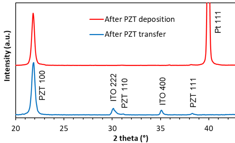
Fig. 2. X-ray Diffraction pattern of the PZT after deposition on Pt/Si (top red plot) and after transfer on glass (bottom blue plot).
