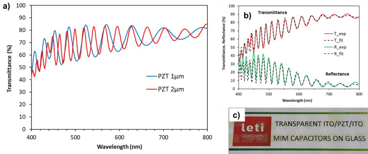
Fig. 4. a) Transmittance spectra of PZT 1 \mu\text{m} and 2 \mu\text{m} , b) Transmittance and reflectance spectra of PZT 2 \mu\text{m} with top ITO layer (experimental and simulation data), c) Photograph of logo and text through transparent PZT capacitors.
