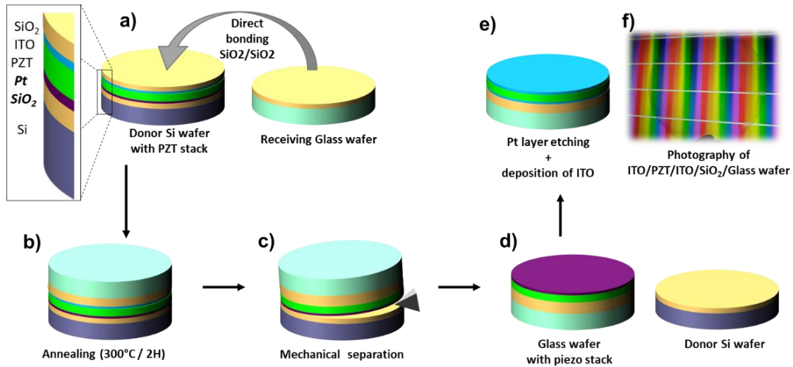
Fig. 1. PZT layer transfer process from Si to glass
