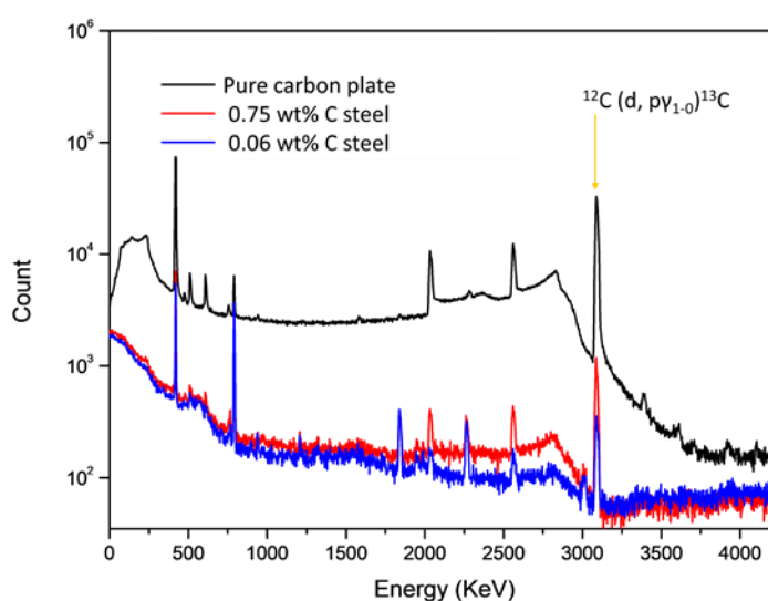
Fig. 3 Gamma spectra from pure carbon sample and two of reference sample excited by deuterium ion beam in He. The yellow arrow shows the gamma peak from carbon in reaction ^{12}\text{C} (d, p\gamma_{1-0})^{13}\text{C}
