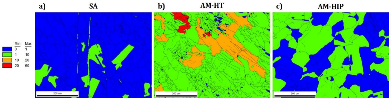
Figure 2: EBSD maps of the misorientation inside the grains also called the Grain Orientation Spread (GOS) for: (a) the cold-rolled SA, (b) the additive manufacturing 316L after heat treatment, AM-HT and (c) after hot isostatic pressure treatment, AM-HIP.
