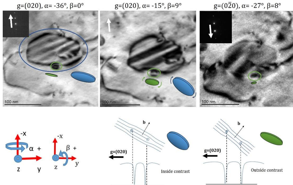
Figure 8: TEM micrographs of the AM HT 316L ASS after 3 dpa ion-irradiation at 550 °C taking in kinematic bright field conditions for (020) and (0 \bar{2} 0). The white arrows on the images show the sense of diffraction vector and the diffraction patterns are in the corner of images. The rotation sense of the \alpha tilt (when \alpha increases) and the rotation sense of the \beta tilt are indicated below TEM images. The orientation and nature of the two loops circled in blue and green are illustrated below the TEM images. The loop circled in blue is an interstitial type loop and the one circled in green is a vacancy-type loop.
