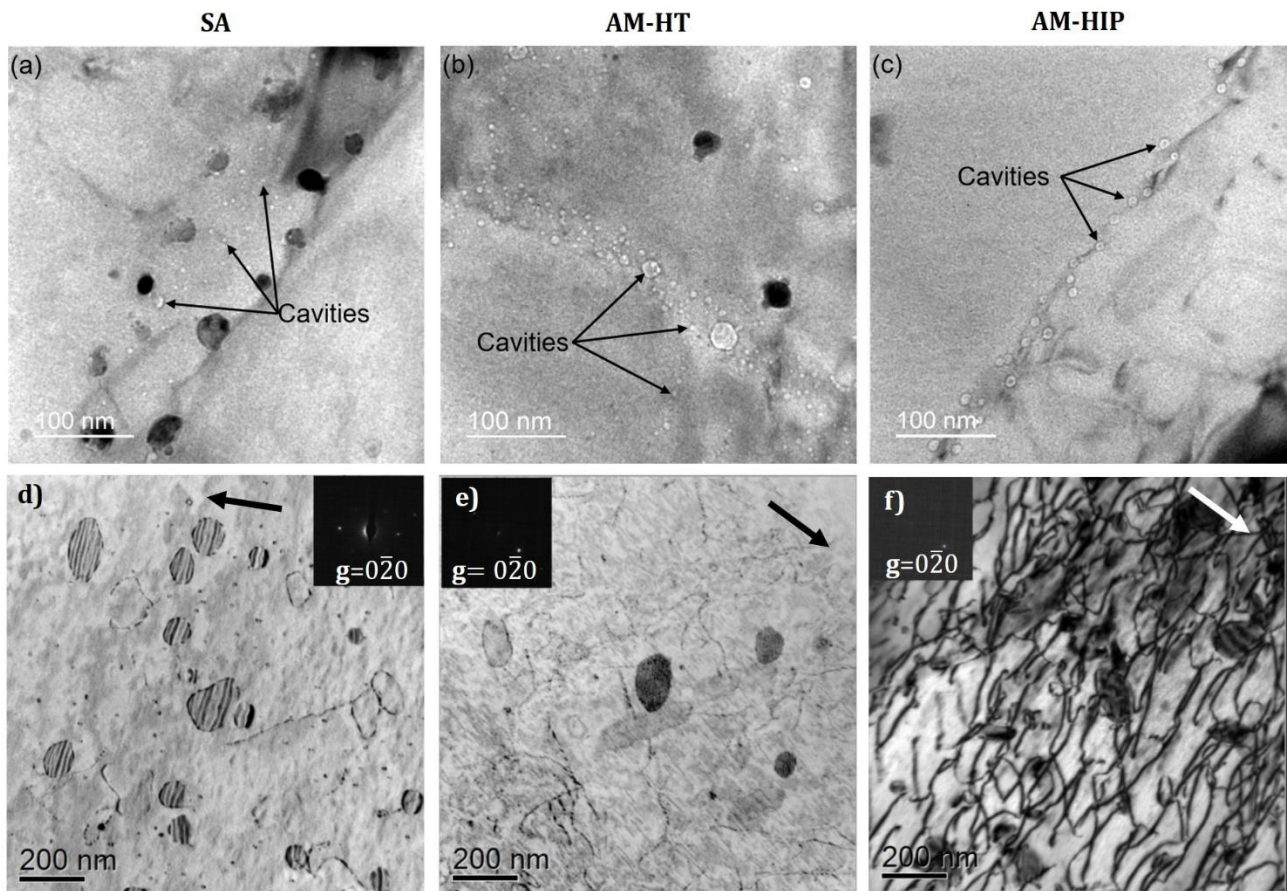
Figure 3: TEM micrographs of: (a, d) SA, (b, e) AM-HT, (c, f) AM-HIP 316L materials after 3 dpa irradiation, showing segregation of cavities at grain boundaries (a-c) and dislocation lines and loops (d-f).
