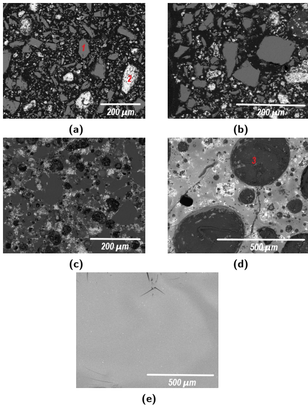
Figure 3: SEM images of the sample at different temperatures ((a) T=300 °C, (b) T=450 °C, (c) T=650 °C, (d) T=800 °C, (e) T=1200 °C) during heating process at 10^{\circ}\text{C}/\text{min} . 1 denotes a grain of glass frit, 2 denotes a grain of calcine and 3 the mark of the bubbles.
