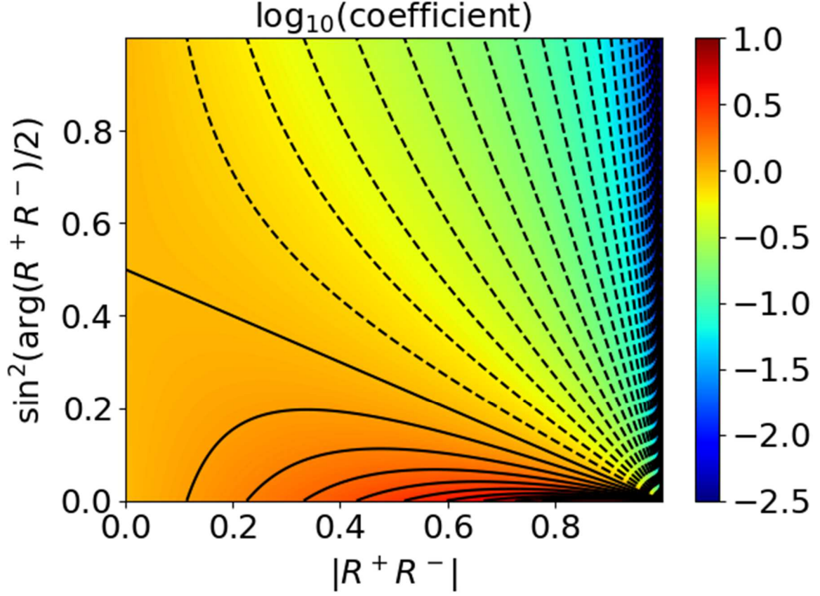
FIGURE 6. Colourmap (log. scale) together with contour lines of the multiplication factor for the total dissipated power (formula (4.15)) versus |R^+R^-| and \sin^2(\arg(R^+R^-)/2) . The straight line corresponds to factor 1 (equation (4.16)).
