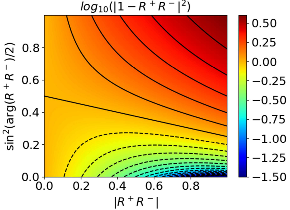
FIGURE 5. Colour map (log. scale) of |1 - R^+ R^-|^2 versus |R^+ R^-| and \sin^2(\arg(R^+ R^-)/2) , together with contour lines. The straight line corresponds to |1 - R^+ R^-| = 1 (equation (4.9)), the dashed curves are contour lines for |1 - R^+ R^-|^2 < 1 .
