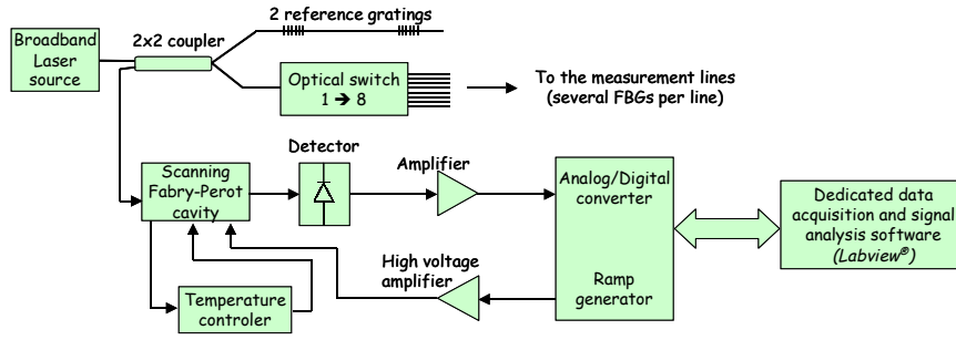
Fig. 5: CEA FBG measurement system architecture
