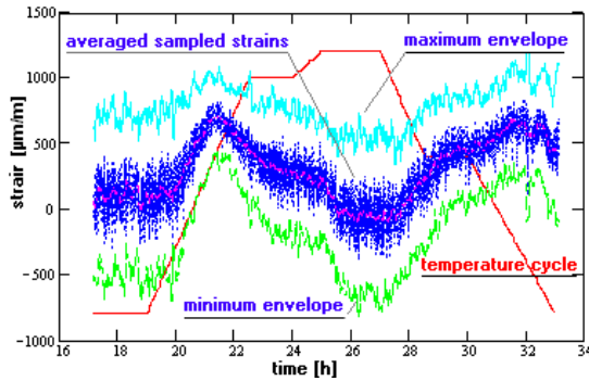
Fig 10: Dynamic fatigue test results (sensor \epsilon_1 )
