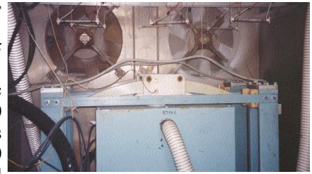
Fig. 8: Experimental set up for fatigue testing
