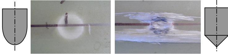
Fig. 7: Cylindrical projectile test and related impact
