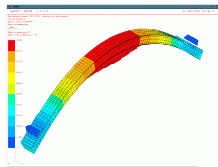
Fig. 4: Static test – FEM – deflection under 150 kN (measured value during test: 72.6 mm)
