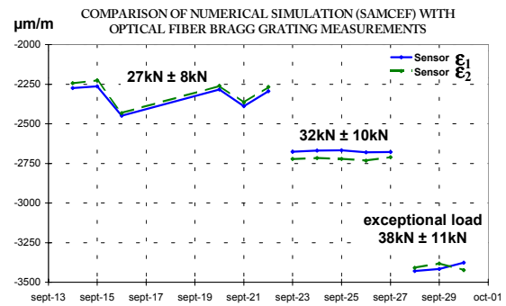
Fig. 11: Strain measurement versus time
