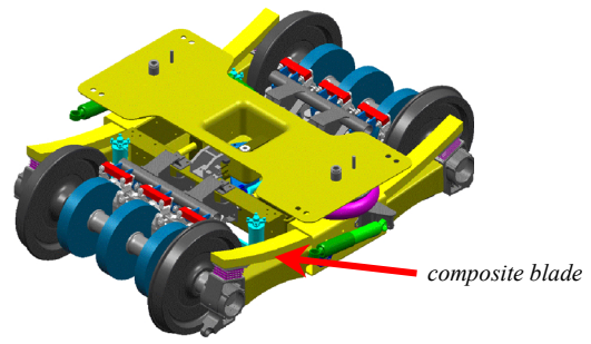
Fig. 3: New Alstom® composite bogie
