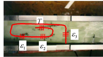
Fig. 9: FBG location inside the composite blade
