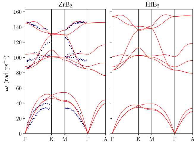
FIG. 2. Phonon dispersion of \text{ZrB}_2 and \text{HfB}_2 . The calculations (lines) are compared with the available experiments (dots) for \text{ZrB}_2(0001) surface phonons [38].
