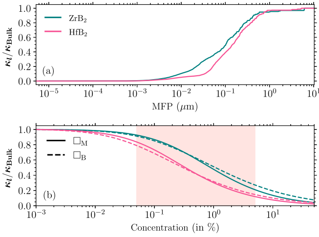
FIG. 5. Variation of \kappa_l/\kappa_{Bulk} at 300 K (a) with respect to phonon mean free path (MFP) contributions, and (b) as a function of defect concentration.
