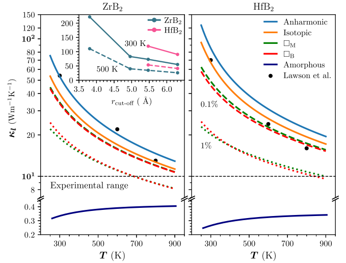
FIG. 3. \kappa_l variation with T for \text{ZrB}_2 and \text{HfB}_2 including different phonon scattering contributions. 0.1% and 1% defect concentrations are considered to elucidate the similar effect of \square_M and \square_B defects over a range of temperatures. Our results are compared with previous calculations by Lawson et al. [6] and a general experimental range of lattice part of thermal conductivity found in most of the literature [7,21] (excluding outliers [20]). Inset shows \kappa_l convergence for \text{ZrB}_2 and \text{HfB}_2 with respect to the IFC cut-off radius ( r_{\text{cut-off}} ).
