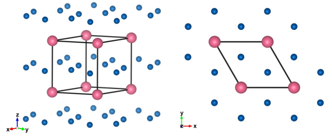
FIG. 1. Side and top view of MB 2 hexagonal crystal structure (space group P6/mmm ). The structure has stacked up alternate layers of metal (pink) and boron (blue) atoms.
