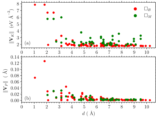
FIG. 6. Squared- L_2 norm of the perturbations (a) IFCs ( \mathbf{V}_K ) and (b) atomic positions ( \mathbf{V}_P ) with reference to the distance from the vacancy ( d ) for \square_M and \square_B vacancies respectively in \text{ZrB}_2 . Strong, short ranged IFC perturbations are seen for \square_B , in contrast to weaker, long-ranged perturbations for \square_M . Similar trends are seen for \text{HfB}_2 in the SM [46].
