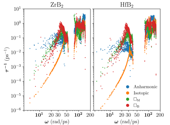
FIG. 4. Phonon scattering contributions from other phonons at 300 K, natural isotopes and vacancy defects in \text{ZrB}_2 and \text{HfB}_2 as a function of \omega . Vacancy concentration of 1% is considered here for both \square_M and \square_B .
