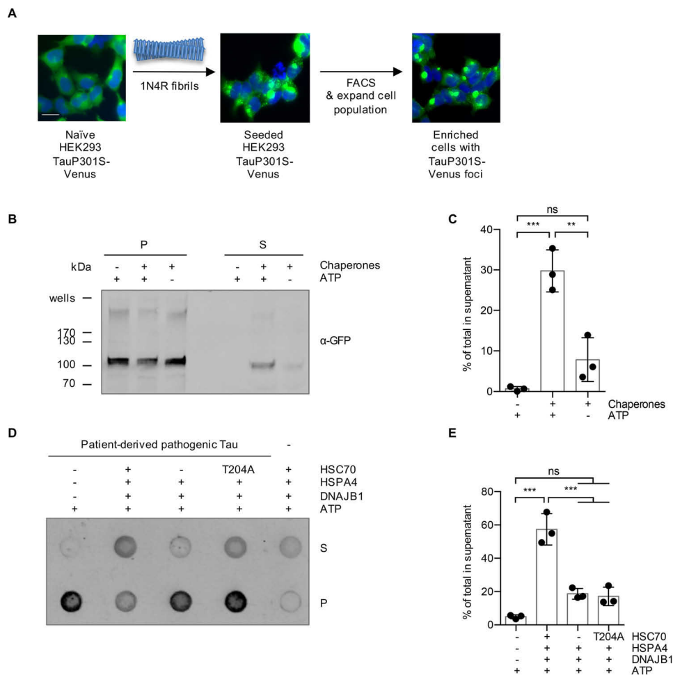
Figure 3. Sarkosyl-insoluble TauP301S-Venus aggregated in a cell culture model and Tau aggregates extracted from AD brain are substrates for the disaggregation machinery. A, a HEK293 0N4R TauP301S-Venus cell line was used to generate a cell population with Tau aggregates as outlined in the depicted workflow. Naïve cells were seeded with 1N4R fibrils, followed by the enrichment of focus-containing cells by FACS. A representative image of the seeded cell population after the FACS enrichment is shown. Scale bar, 20 \mu m. B, Sarkosyl-insoluble TauP301S-Venus material extracted from the seeded HEK293 cell population was subjected to in vitro disaggregation assays with the recombinant human Hsp70 disaggregation machinery (HSC70, DNAJB1, HSPA4) \pm ATP for 20 h at 30 ^{\circ} C. S and P fractions were separated by centrifugation at 337,000 \times g and analyzed by immunoblotting with an \alpha -GFP antibody detecting TauP301S-Venus. C, densitometric quantification of TauP301S-Venus in S fractions compared with the total (S + P) of the Western blot shown in panel B. n = 3 , mean \pm S.D. One-way ANOVA with Bonferroni's multiple comparison test. ns, not significant; ***, p \leq 0.001 . D, the Sarkosyl-insoluble fraction extracted from an AD brain was subjected to in vitro disaggregation assays for 20 h at 30 ^{\circ} C. The samples were treated either with the complete disaggregation machinery (HSC70, DNAJB1, HSPA4), with only DNAJB1 and HSPA4, omitting HSC70, or with DNAJB1 and HSPA4 together with an ATPase-defective mutant HSC70 (T204A). S and P fractions were separated by centrifugation at 150,000 \times g and analyzed by dot blotting with the \alpha -Tau antibody HT7. E, densitometric quantification of the dot blot shown in panel D. The percentage of Tau in S fractions compared with the total (S + P) was calculated for each sample. The background signal of chaperones without patient material was subtracted. n = 3 , mean \pm S.D. One-way ANOVA with Bonferroni's multiple comparison test was used. ns, not significant; ***, p \leq 0.001 .
