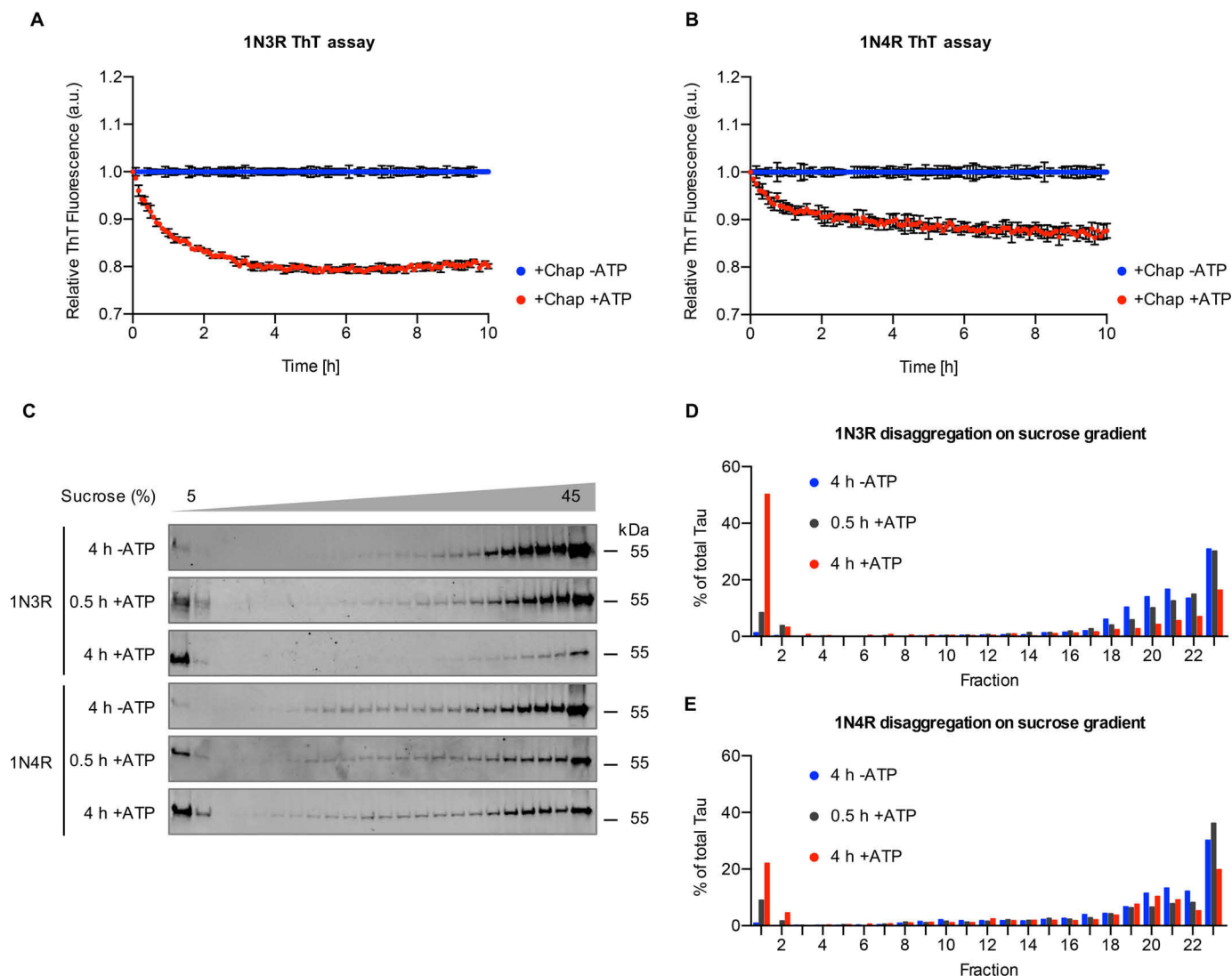
Figure 5. The disaggregation reaction generates low-molecular-weight species. A and B, 1N3R (A) and 1N4R (B) Tau fibrils were treated with chaperones in the presence or absence of ATP. Thioflavin T (ThT) fluorescence was monitored over time as a readout of amyloid content. Per condition, three independent disaggregation reactions were measured ( n = 3 , mean \pm S.D.). C, Tau fibrils were treated with the disaggregation machinery for 30 min or 4 h at 30 °C and subsequently centrifuged over a 5–45% sucrose gradient. Representative blots of three (1N3R) and two (1N4R) replicates are shown. Fractions were collected manually, and Tau levels were analyzed by immunoblotting. D and E, densitometric quantification of 1N3R disaggregation (D) and 1N4R disaggregation (E) of the experiment shown in panel C. The amount in each fraction was calculated as a percentage of the total amount of Tau in all fractions.
