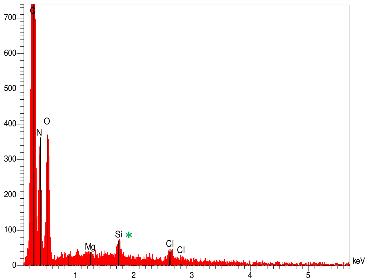
Figure 19: EDS analysis of a washed C 2 N sample (star : signal from the substrate).
