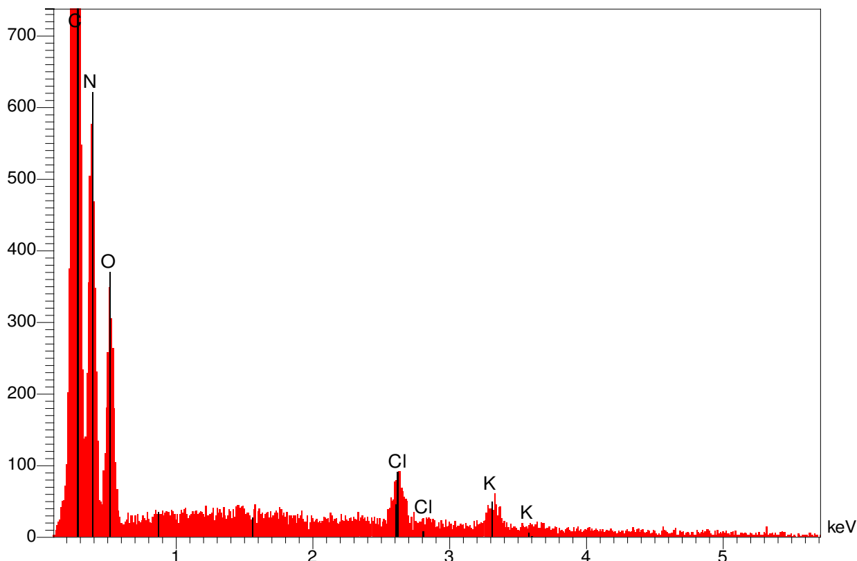
Figure 7. EDS analysis of CN.
