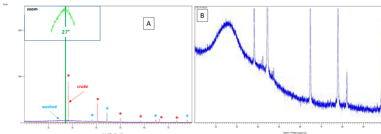
Figure 16 : A) compared powder X-ray diffractograms of a crude (red) and washed (blue) C 2 N samples (same batch). Insert (green): zoom over the blue curve. Blue stars : signals from the aluminum sample holder ; red stars : signals from KCl by-product. B) : Powder x-ray diffractogram of the washed C 2 N sample. Black stars : signals from the aluminum sample holder.
